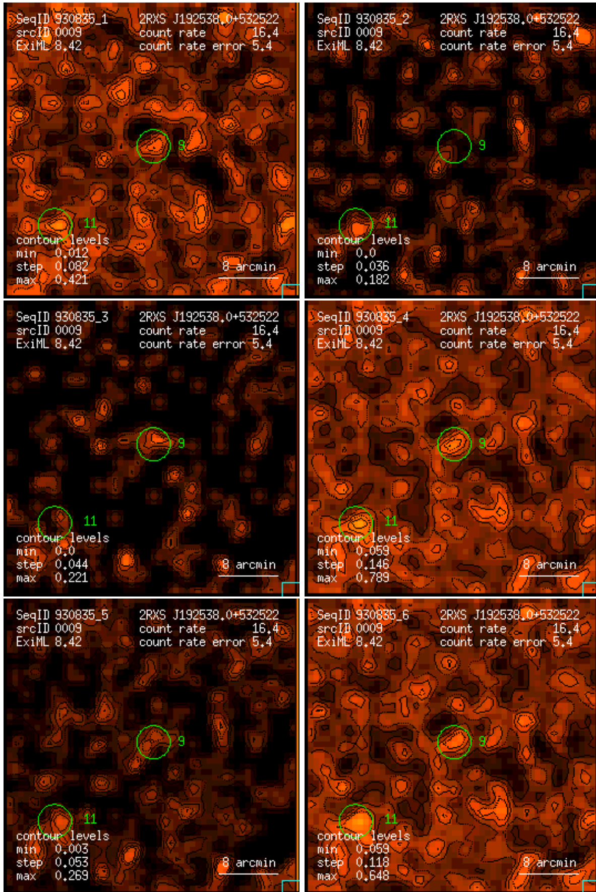
Figure 9: RASS 930835: detection 0009: band rate images, Gaussian filter: (1) PSPC channels 11 – 41, (2) 52 – 90, (3) 91 – 201, (4) 11 – 235, (5) 52 – 201, (6) 11 – 201. Broad band rates in counts/ks. Band rate contour levels in counts/ks/arcmin 2 .
