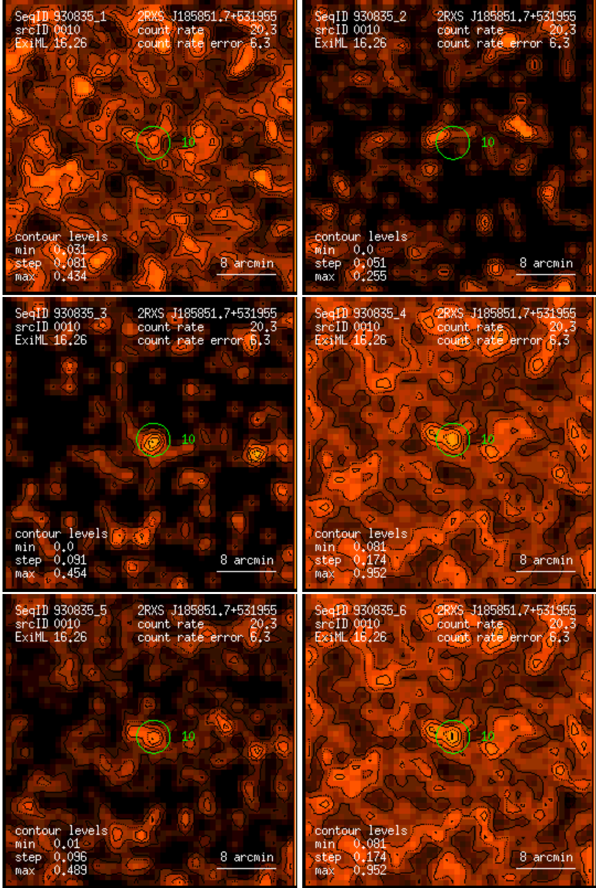
Figure 10: RASS 930835: detection 0010: band rate images, Gaussian filter: (1) PSPC channels 11 – 41, (2) 52 – 90, (3) 91 – 201, (4) 11 – 235, (5) 52 – 201, (6) 11 – 201. Broad band rates in counts/ks. Band rate contour levels in counts/ks/arcmin 2 .
