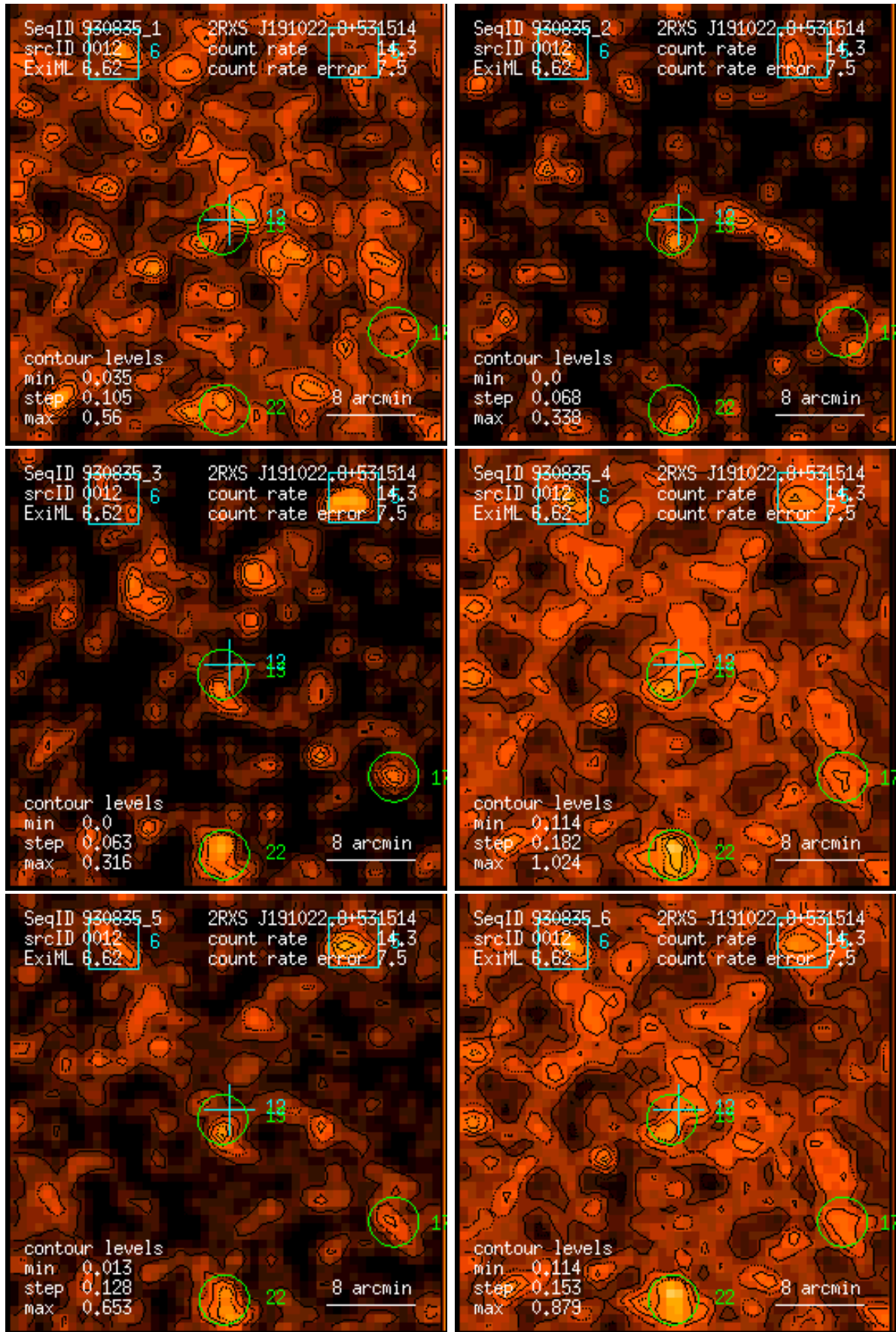
Figure 12: RASS 930835: detection 0012: band rate images, Gaussian filter: (1) PSPC channels 11 – 41, (2) 52 – 90, (3) 91 – 201, (4) 11 – 235, (5) 52 – 201, (6) 11 – 201. Broad band rates in counts/ks. Band rate contour levels in counts/ks/arcmin 2 .
