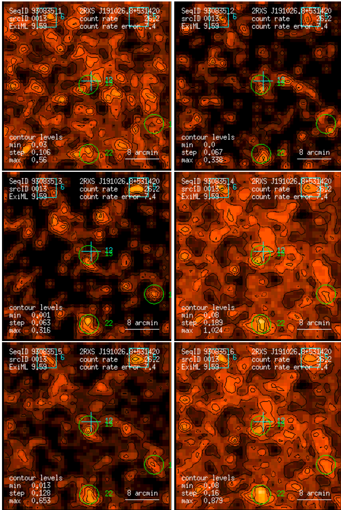
Figure 13: RASS 930835: detection 0013: band rate images, Gaussian filter: (1) PSPC channels 11 – 41, (2) 52 – 90, (3) 91 – 201, (4) 11 – 235, (5) 52 – 201, (6) 11 – 201. Broad band rates in counts/ks. Band rate contour levels in counts/ks/arcmin 2 .
