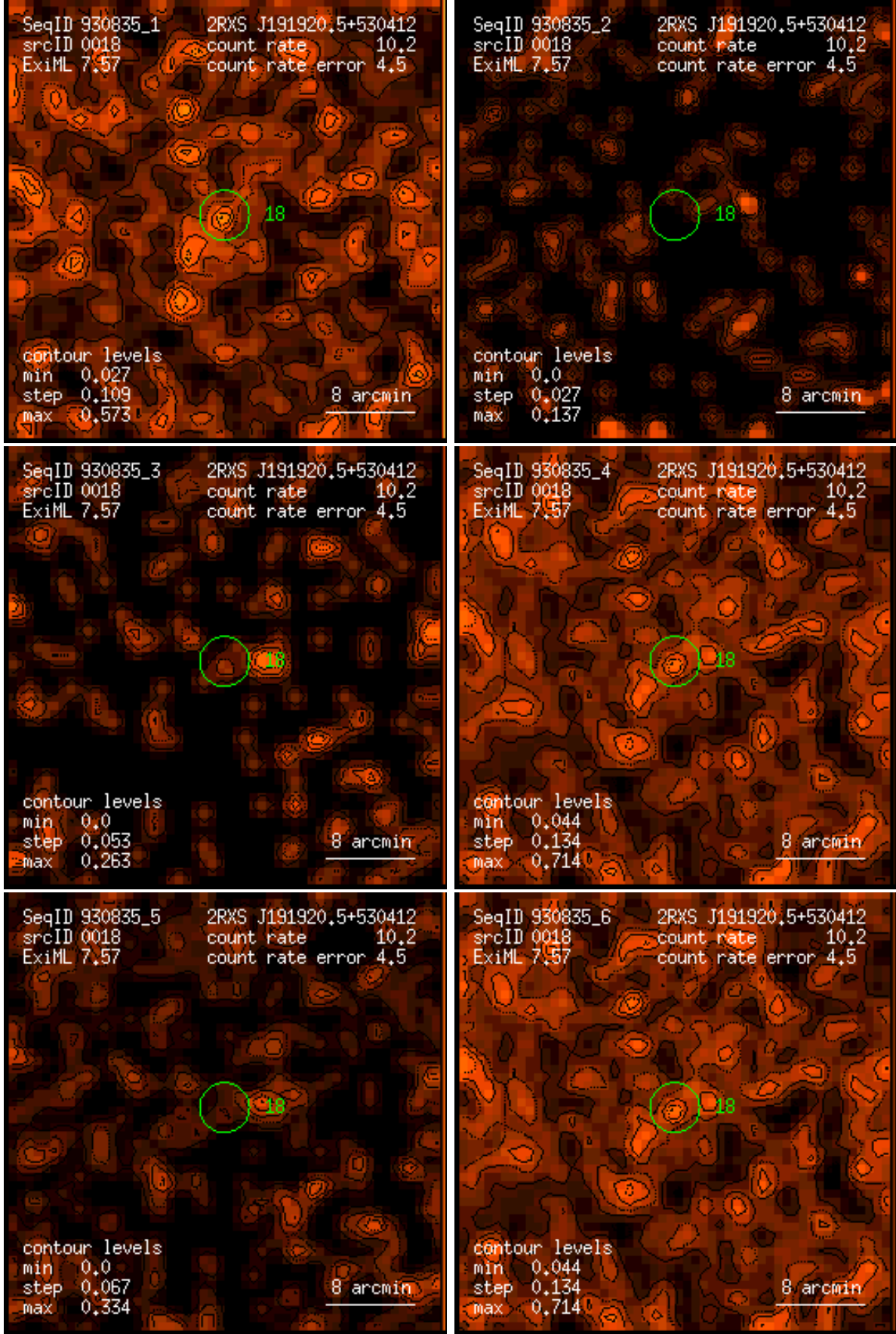
Figure 18: RASS 930835: detection 0018: band rate images, Gaussian filter: (1) PSPC channels 11 – 41, (2) 52 – 90, (3) 91 – 201, (4) 11 – 235, (5) 52 – 201, (6) 11 – 201. Broad band rates in counts/ks. Band rate contour levels in counts/ks/arcmin 2 .
