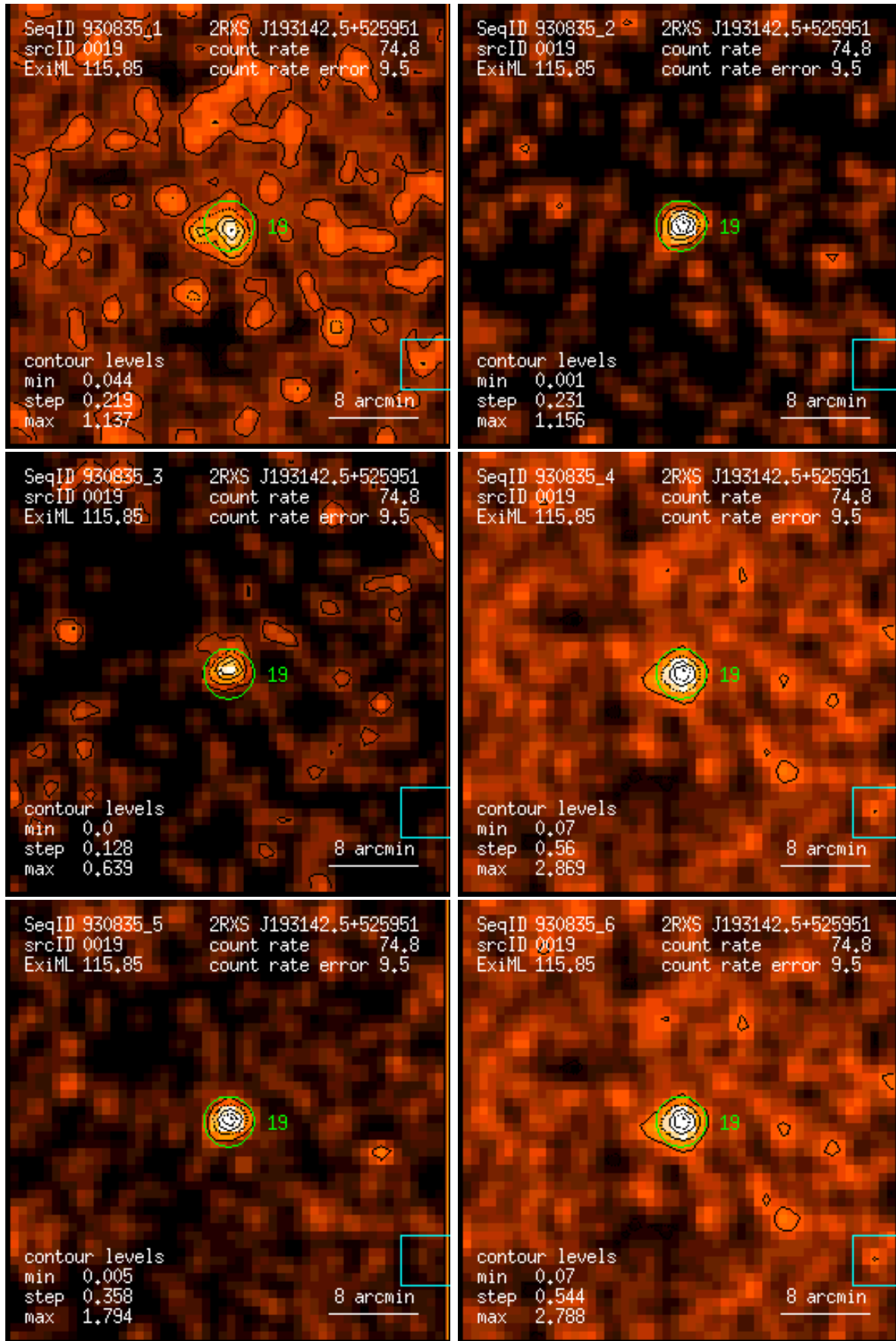
Figure 19: RASS 930835: detection 0019: band rate images, Gaussian filter: (1) PSPC channels 11 – 41, (2) 52 – 90, (3) 91 – 201, (4) 11 – 235, (5) 52 – 201, (6) 11 – 201. Broad band rates in counts/ks. Band rate contour levels in counts/ks/arcmin 2 .
