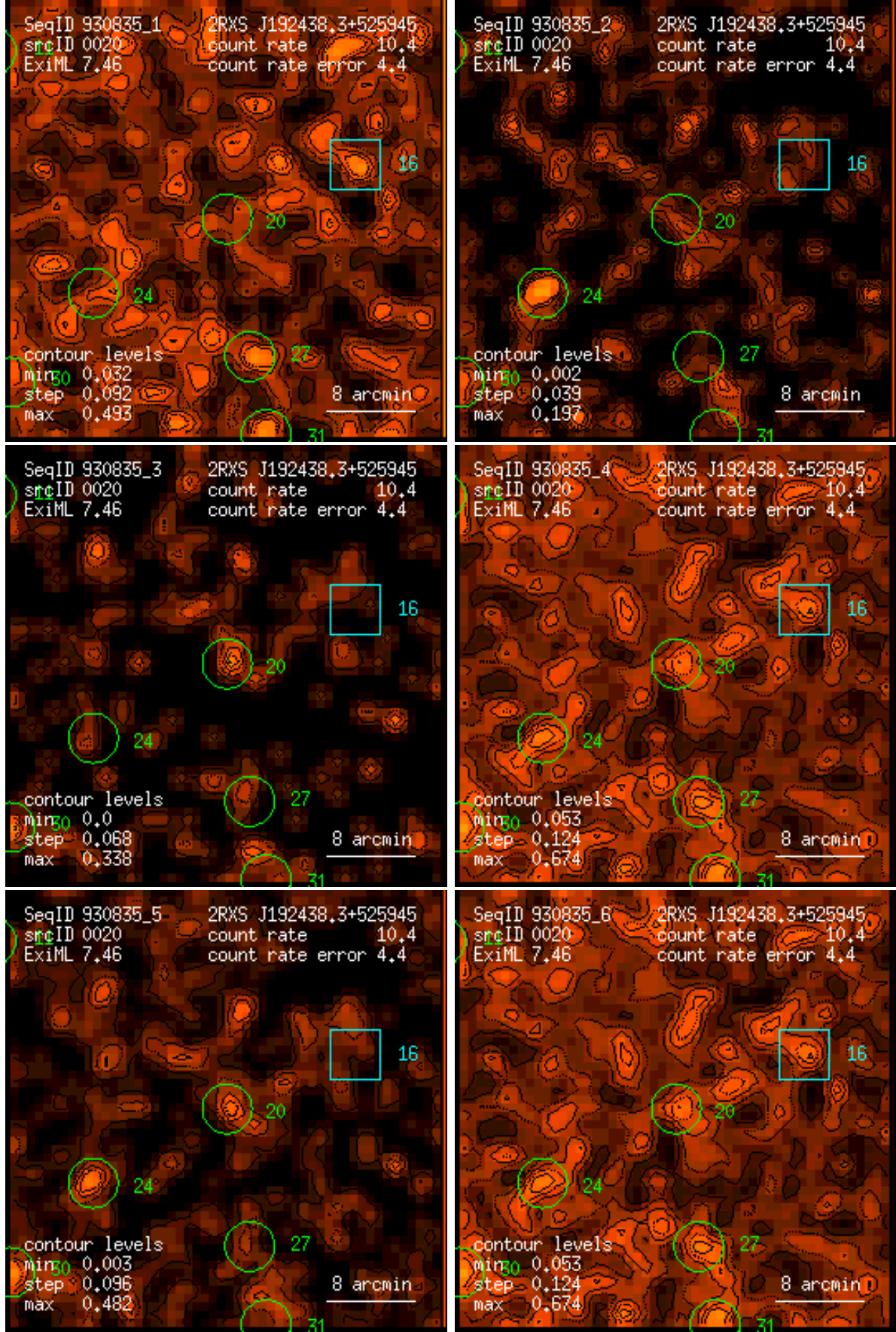
Figure 20: RASS 930835: detection 0020: band rate images, Gaussian filter: (1) PSPC channels 11 – 41, (2) 52 – 90, (3) 91 – 201, (4) 11 – 235, (5) 52 – 201, (6) 11 – 201. Broad band rates in counts/ks. Band rate contour levels in counts/ks/arcmin 2 .
