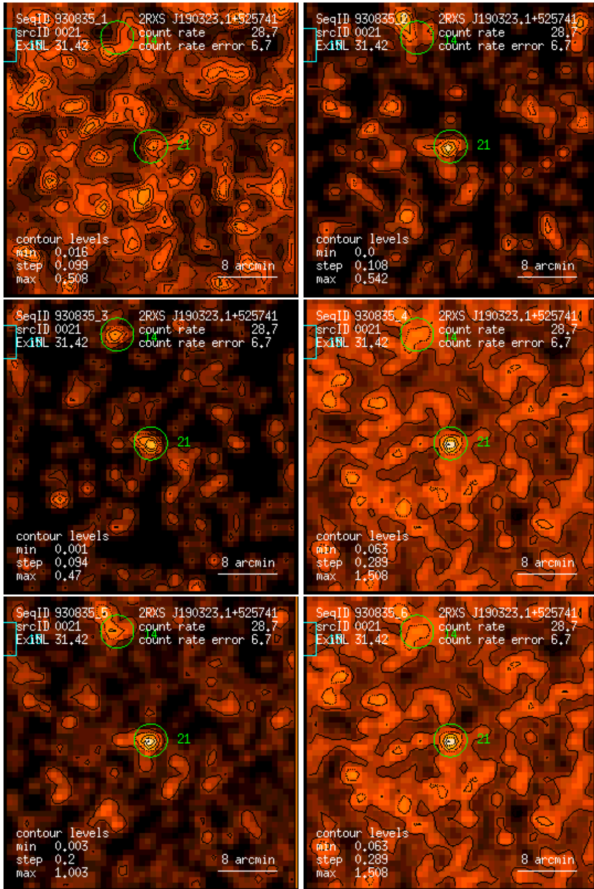
Figure 21: RASS 930835: detection 0021: band rate images, Gaussian filter: (1) PSPC channels 11 – 41, (2) 52 – 90, (3) 91 – 201, (4) 11 – 235, (5) 52 – 201, (6) 11 – 201. Broad band rates in counts/ks. Band rate contour levels in counts/ks/arcmin 2 .
