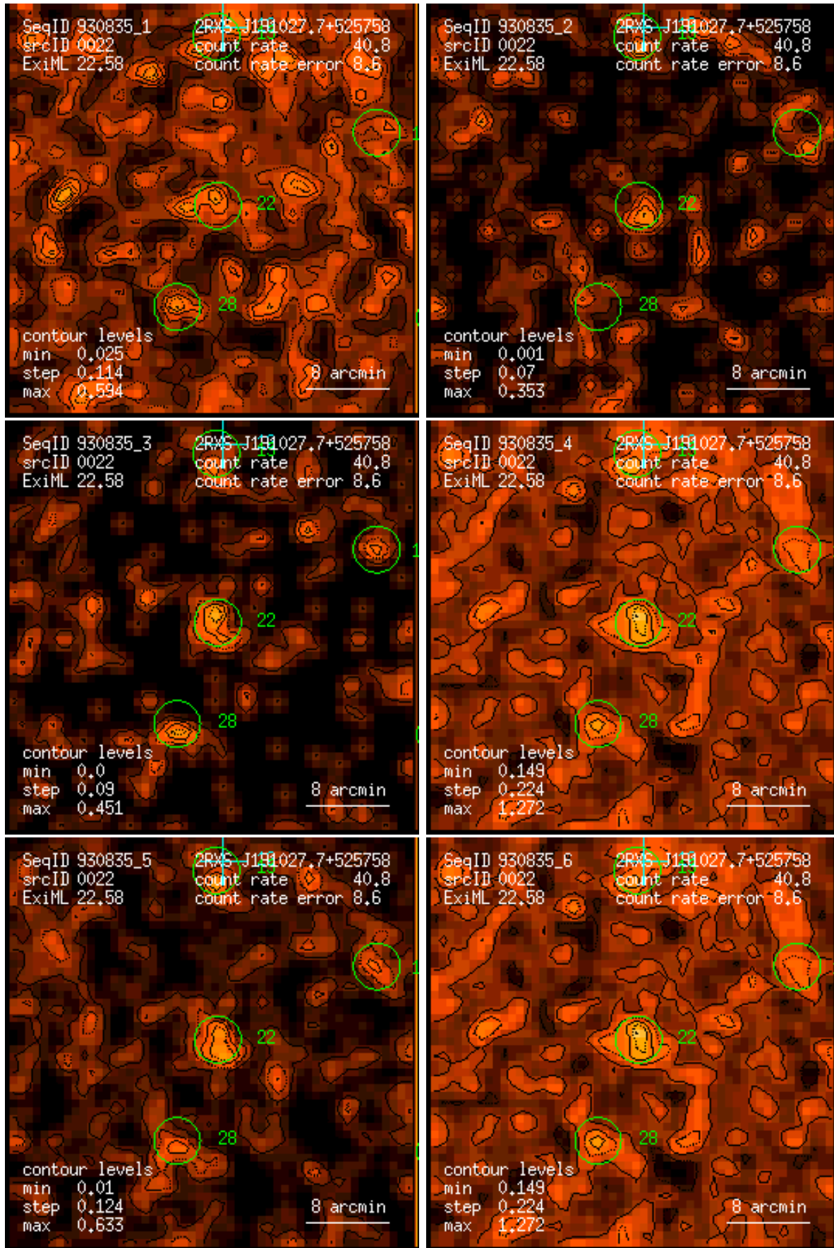
Figure 22: RASS 930835: detection 0022: band rate images, Gaussian filter: (1) PSPC channels 11 – 41, (2) 52 – 90, (3) 91 – 201, (4) 11 – 235, (5) 52 – 201, (6) 11 – 201. Broad band rates in counts/ks. Band rate contour levels in counts/ks/arcmin 2 .
