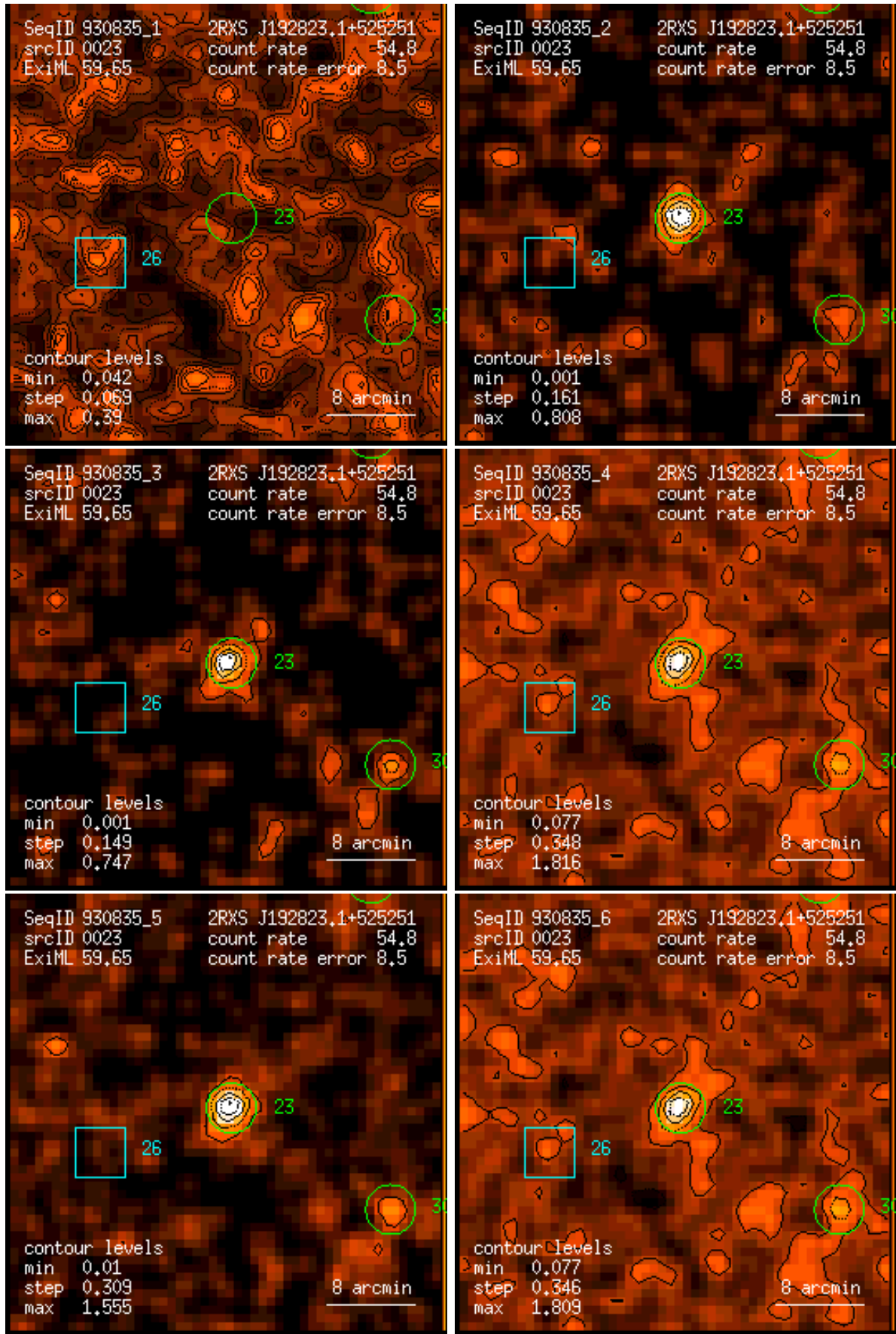
Figure 23: RASS 930835: detection 0023: band rate images, Gaussian filter: (1) PSPC channels 11 – 41, (2) 52 – 90, (3) 91 – 201, (4) 11 – 235, (5) 52 – 201, (6) 11 – 201. Broad band rates in counts/ks. Band rate contour levels in counts/ks/arcmin 2 .
