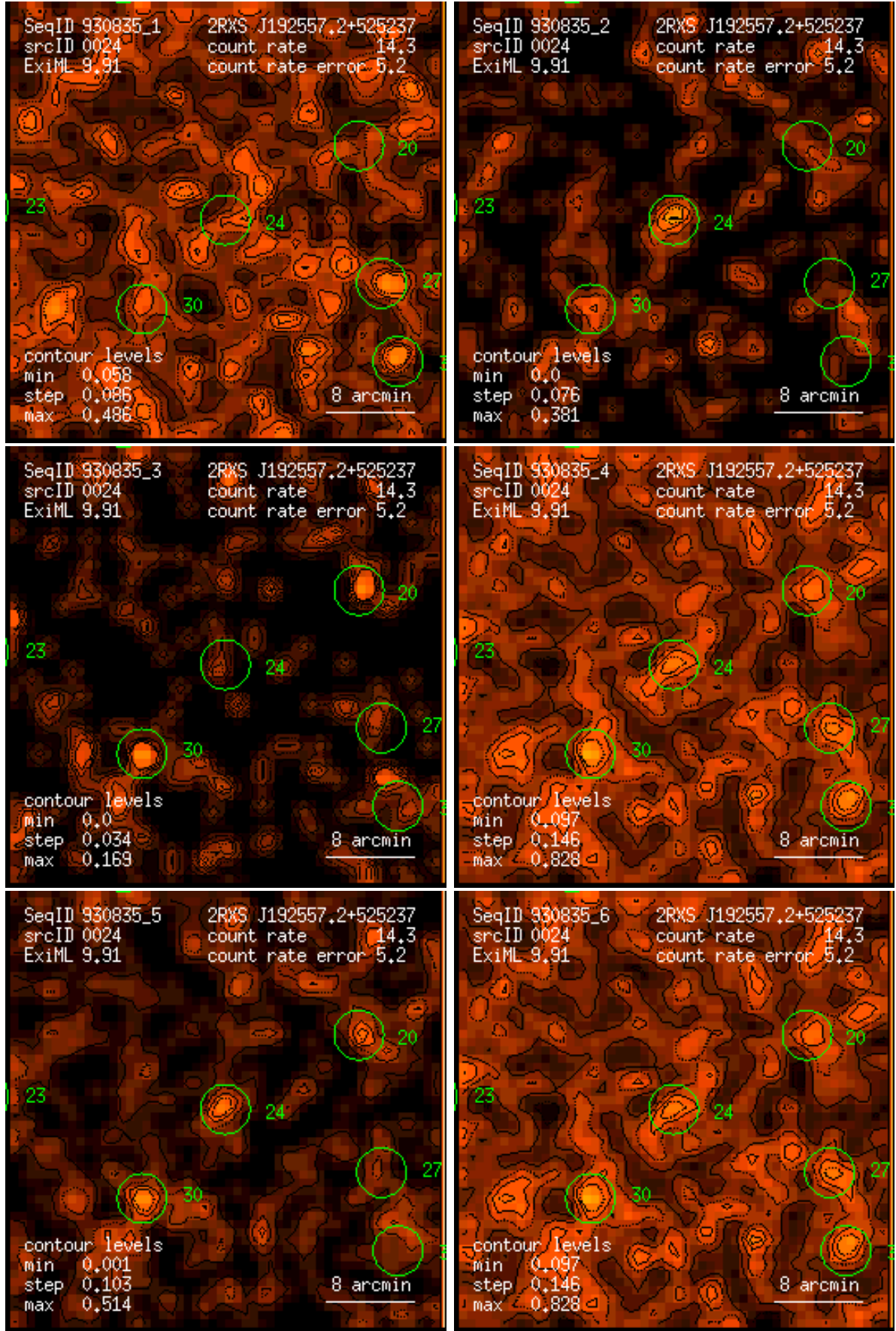
Figure 24: RASS 930835: detection 0024: band rate images, Gaussian filter: (1) PSPC channels 11 – 41, (2) 52 – 90, (3) 91 – 201, (4) 11 – 235, (5) 52 – 201, (6) 11 – 201. Broad band rates in counts/ks. Band rate contour levels in counts/ks/arcmin 2 .
