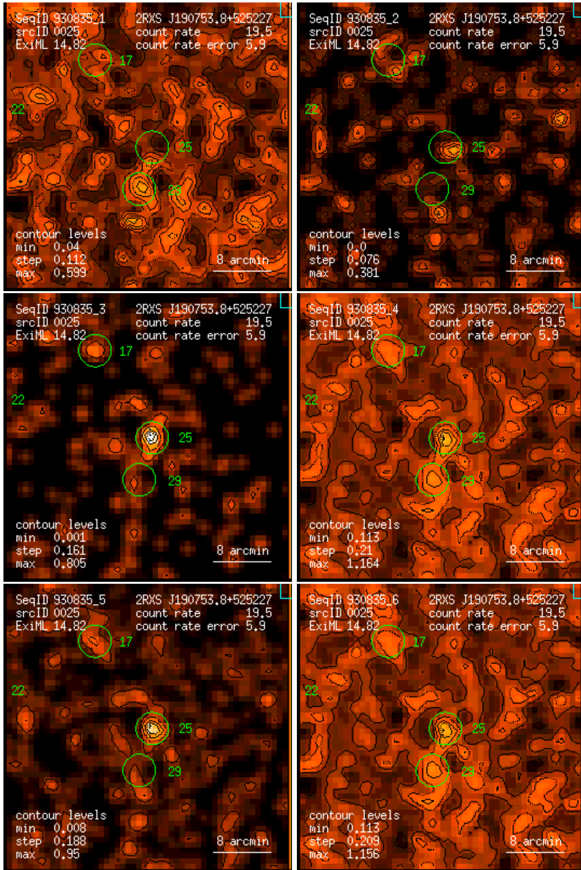
Figure 25: RASS 930835: detection 0025: band rate images, Gaussian filter: (1) PSPC channels 11 – 41, (2) 52 – 90, (3) 91 – 201, (4) 11 – 235, (5) 52 – 201, (6) 11 – 201. Broad band rates in counts/ks. Band rate contour levels in counts/ks/arcmin 2 .
