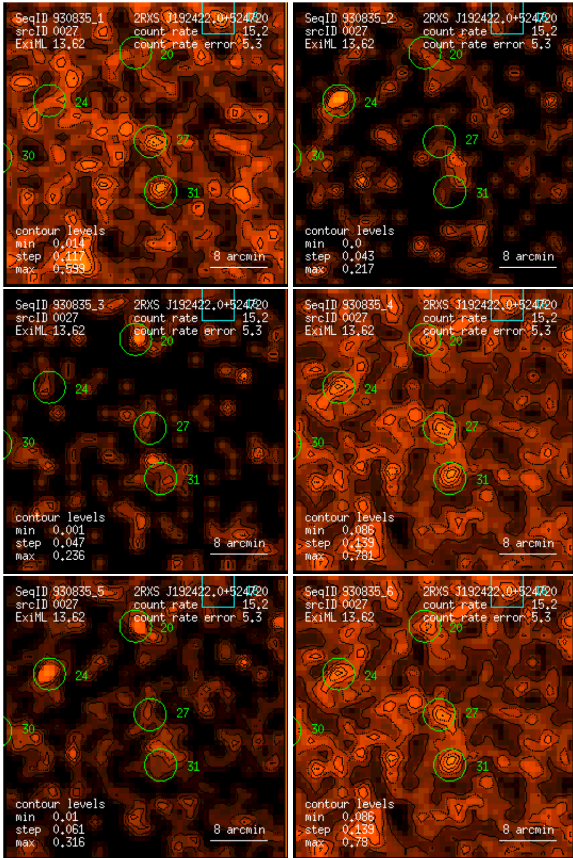
Figure 27: RASS 930835: detection 0027: band rate images, Gaussian filter: (1) PSPC channels 11 – 41, (2) 52 – 90, (3) 91 – 201, (4) 11 – 235, (5) 52 – 201, (6) 11 – 201. Broad band rates in counts/ks. Band rate contour levels in counts/ks/arcmin 2 .
