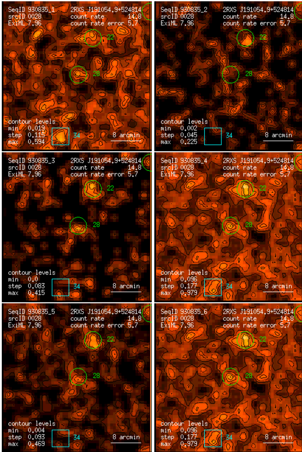
Figure 28: RASS 930835: detection 0028: band rate images, Gaussian filter: (1) PSPC channels 11 – 41, (2) 52 – 90, (3) 91 – 201, (4) 11 – 235, (5) 52 – 201, (6) 11 – 201. Broad band rates in counts/ks. Band rate contour levels in counts/ks/arcmin 2 .
