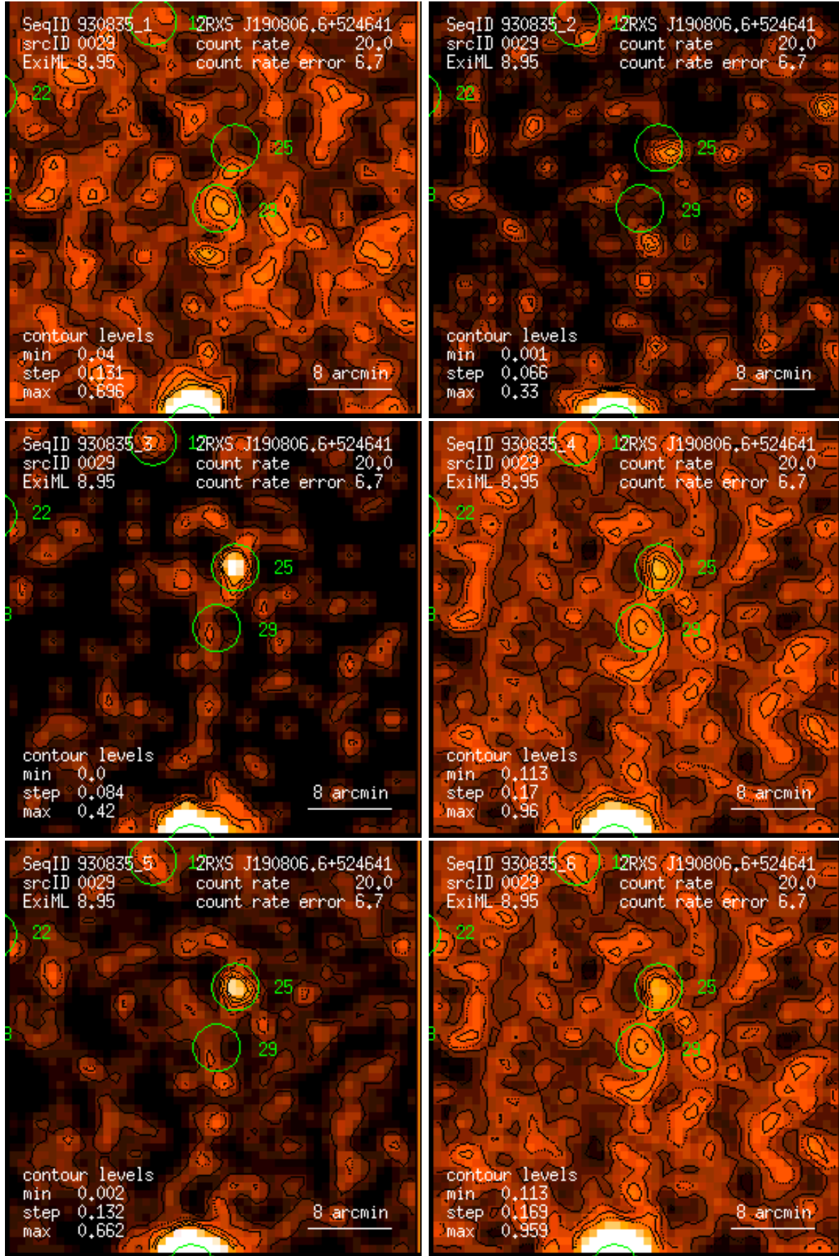
Figure 29: RASS 930835: detection 0029: band rate images, Gaussian filter: (1) PSPC channels 11 – 41, (2) 52 – 90, (3) 91 – 201, (4) 11 – 235, (5) 52 – 201, (6) 11 – 201. Broad band rates in counts/ks. Band rate contour levels in counts/ks/arcmin 2 .
