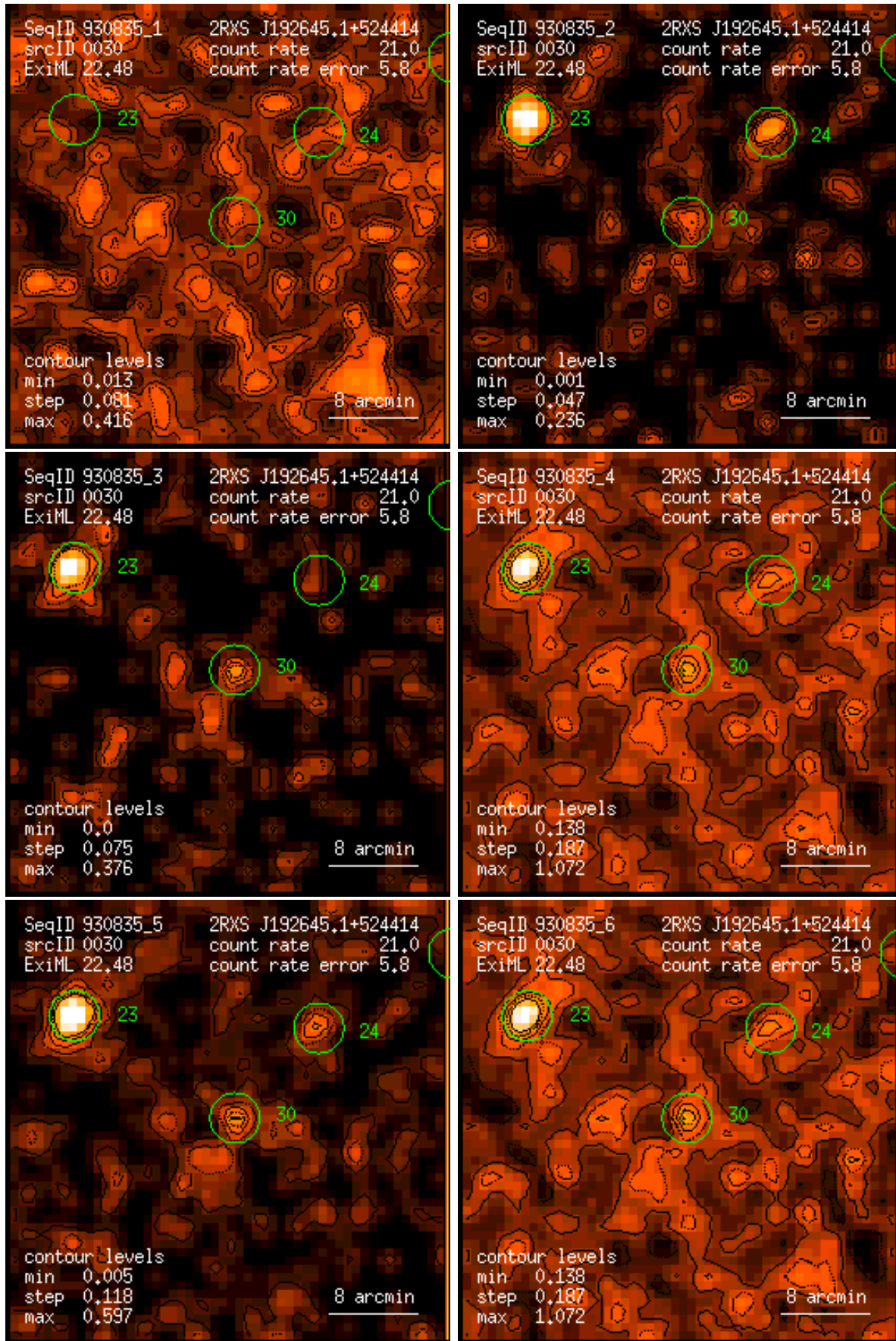
Figure 30: RASS 930835: detection 0030: band rate images, Gaussian filter: (1) PSPC channels 11 – 41, (2) 52 – 90, (3) 91 – 201, (4) 11 – 235, (5) 52 – 201, (6) 11 – 201. Broad band rates in counts/ks. Band rate contour levels in counts/ks/arcmin 2 .
