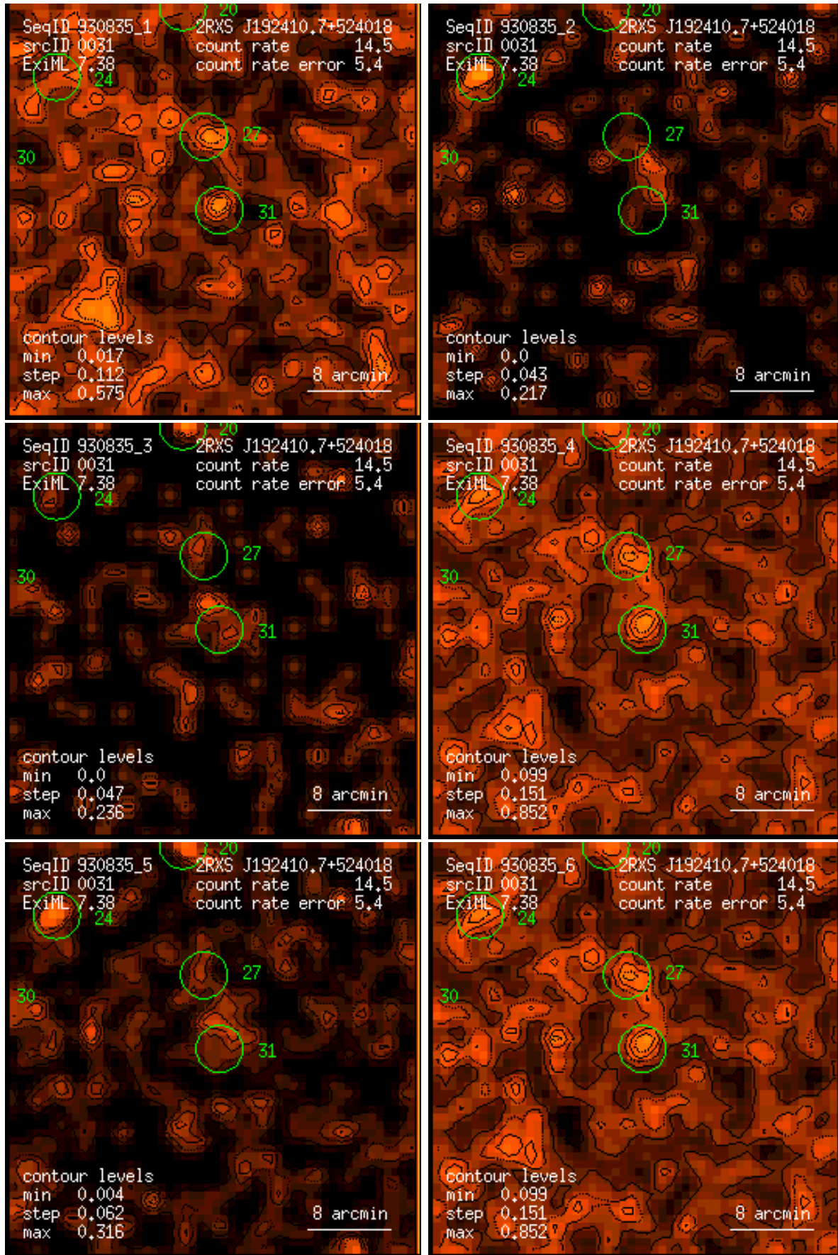
Figure 31: RASS 930835: detection 0031: band rate images, Gaussian filter: (1) PSPC channels 11 – 41, (2) 52 – 90, (3) 91 – 201, (4) 11 – 235, (5) 52 – 201, (6) 11 – 201. Broad band rates in counts/ks. Band rate contour levels in counts/ks/arcmin 2 .
