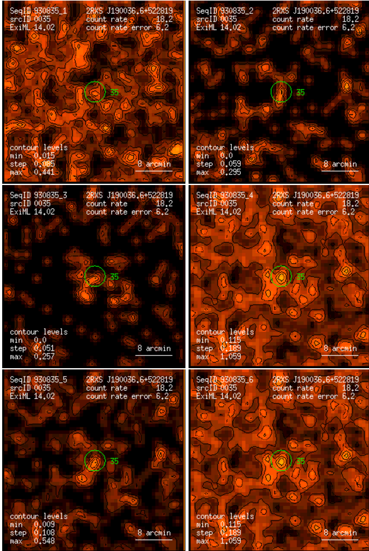
Figure 35: RASS 930835: detection 0035: band rate images, Gaussian filter: (1) PSPC channels 11 – 41, (2) 52 – 90, (3) 91 – 201, (4) 11 – 235, (5) 52 – 201, (6) 11 – 201. Broad band rates in counts/ks. Band rate contour levels in counts/ks/arcmin 2 .
