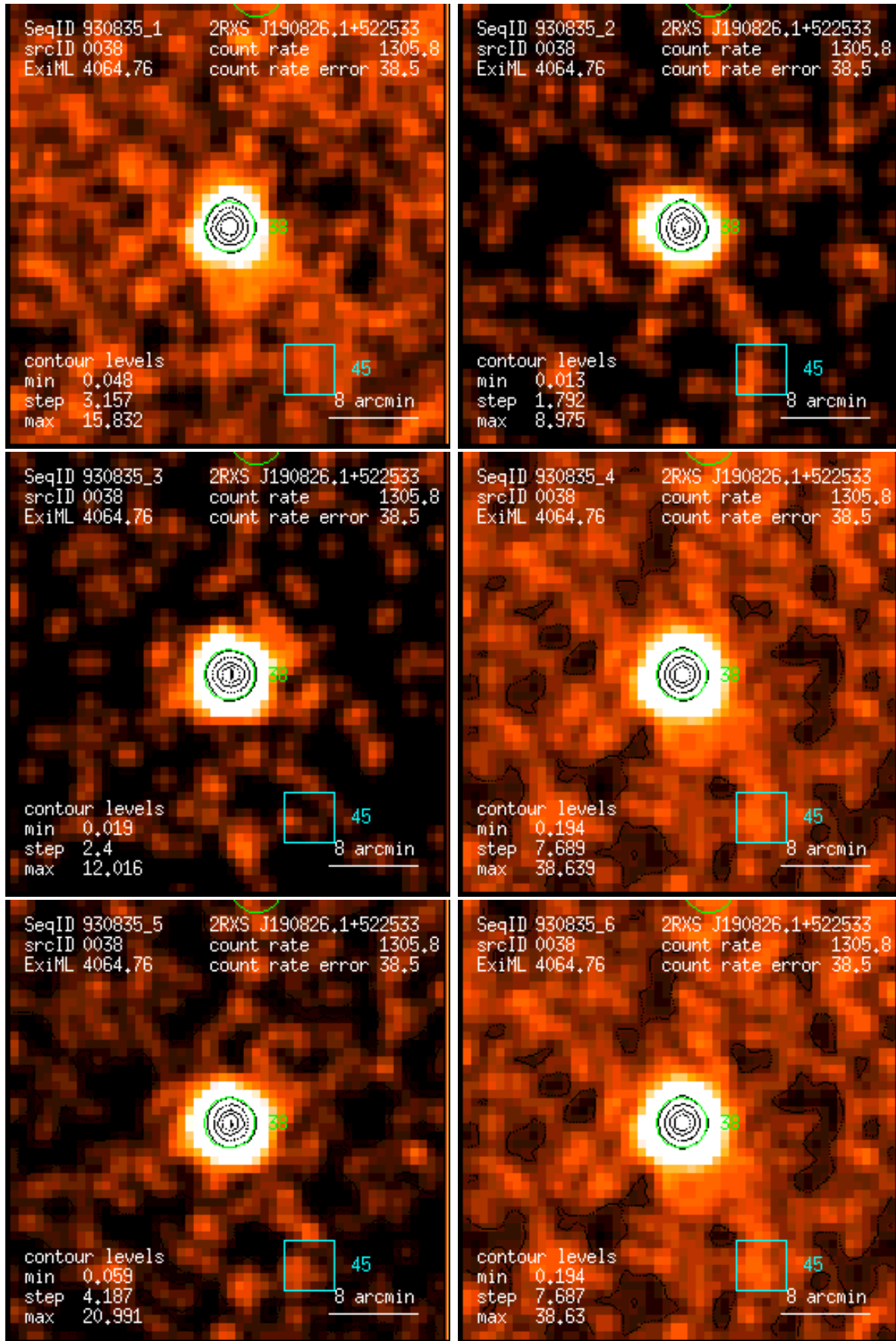
Figure 38: RASS 930835: detection 0038: band rate images, Gaussian filter: (1) PSPC channels 11 – 41, (2) 52 – 90, (3) 91 – 201, (4) 11 – 235, (5) 52 – 201, (6) 11 – 201. Broad band rates in counts/ks. Band rate contour levels in counts/ks/arcmin 2 .
