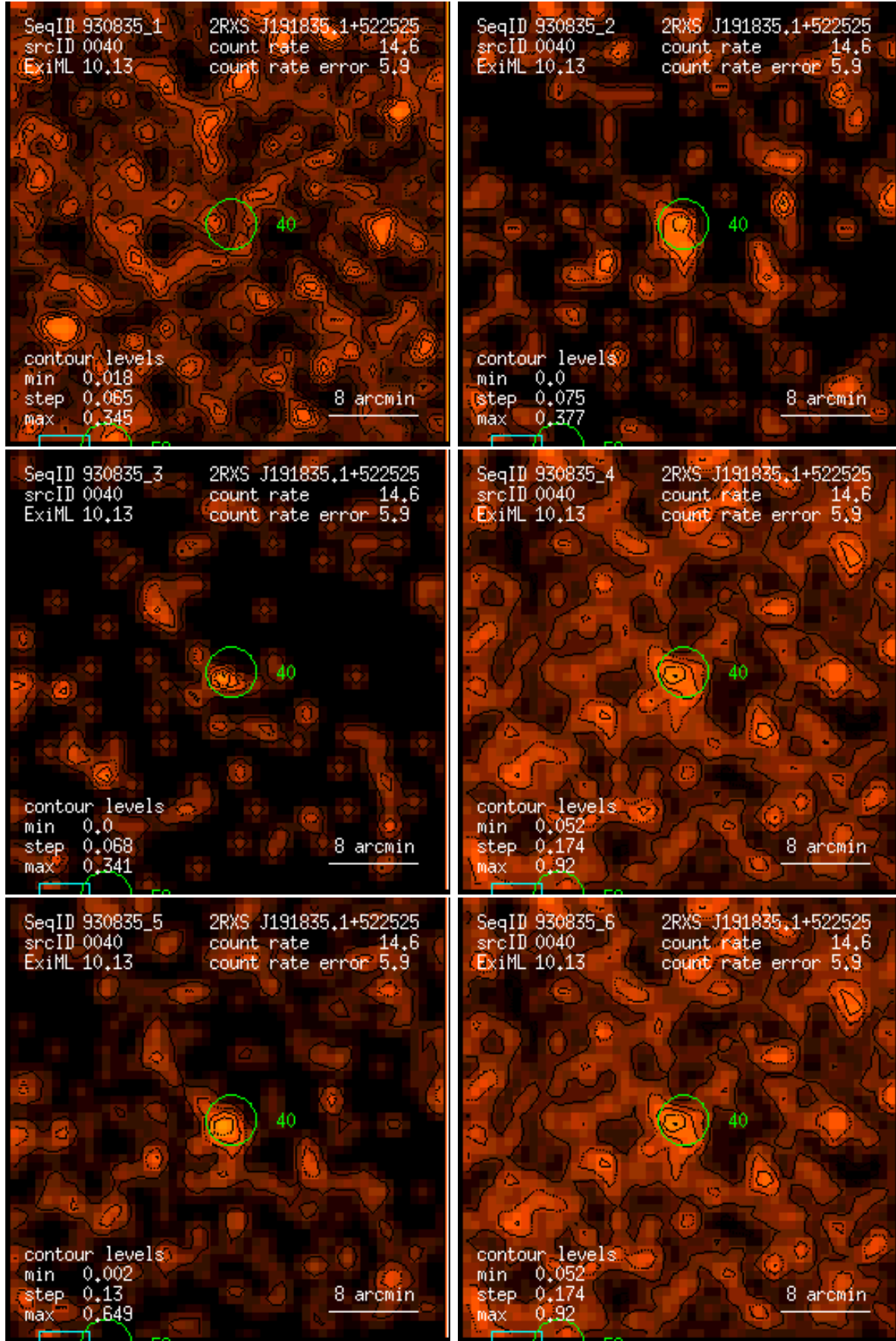
Figure 40: RASS 930835: detection 0040: band rate images, Gaussian filter: (1) PSPC channels 11 – 41, (2) 52 – 90, (3) 91 – 201, (4) 11 – 235, (5) 52 – 201, (6) 11 – 201. Broad band rates in counts/ks. Band rate contour levels in counts/ks/arcmin 2 .
