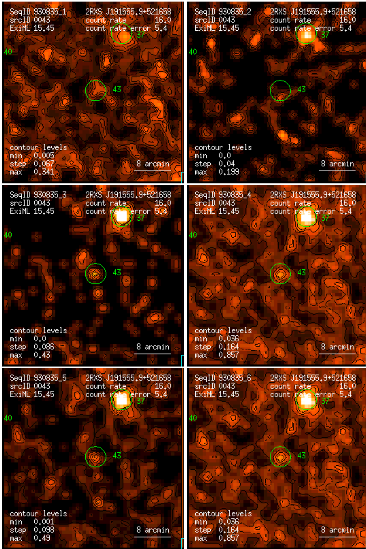
Figure 43: RASS 930835: detection 0043: band rate images, Gaussian filter: (1) PSPC channels 11 – 41, (2) 52 – 90, (3) 91 – 201, (4) 11 – 235, (5) 52 – 201, (6) 11 – 201. Broad band rates in counts/ks. Band rate contour levels in counts/ks/arcmin 2 .
