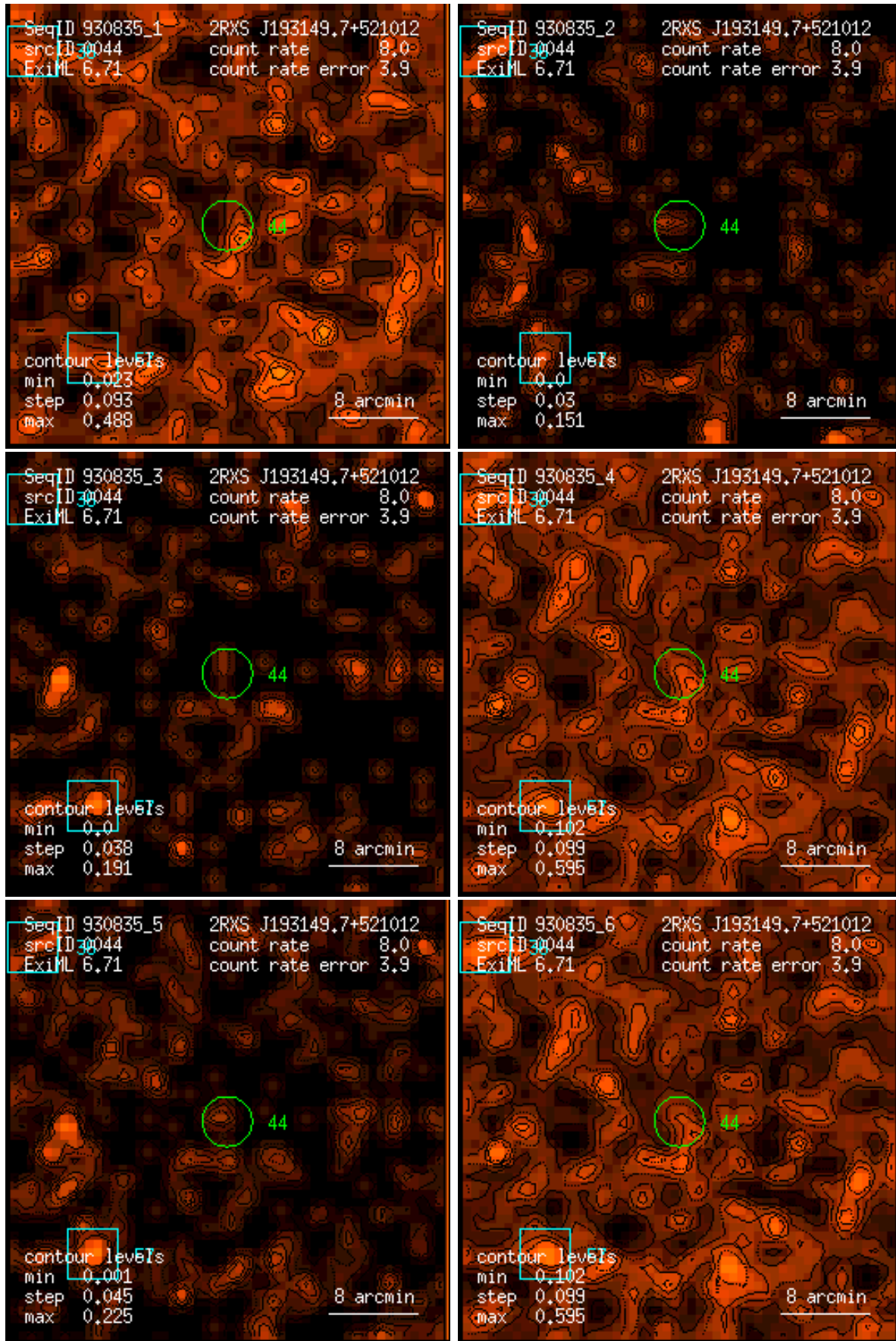
Figure 44: RASS 930835: detection 0044: band rate images, Gaussian filter: (1) PSPC channels 11 – 41, (2) 52 – 90, (3) 91 – 201, (4) 11 – 235, (5) 52 – 201, (6) 11 – 201. Broad band rates in counts/ks. Band rate contour levels in counts/ks/arcmin 2 .
