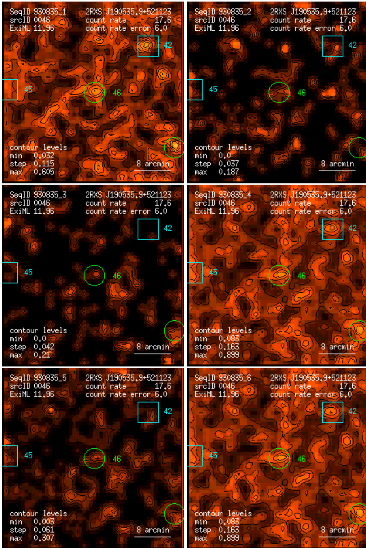
Figure 46: RASS 930835: detection 0046: band rate images, Gaussian filter: (1) PSPC channels 11 – 41, (2) 52 – 90, (3) 91 – 201, (4) 11 – 235, (5) 52 – 201, (6) 11 – 201. Broad band rates in counts/ks. Band rate contour levels in counts/ks/arcmin 2 .
