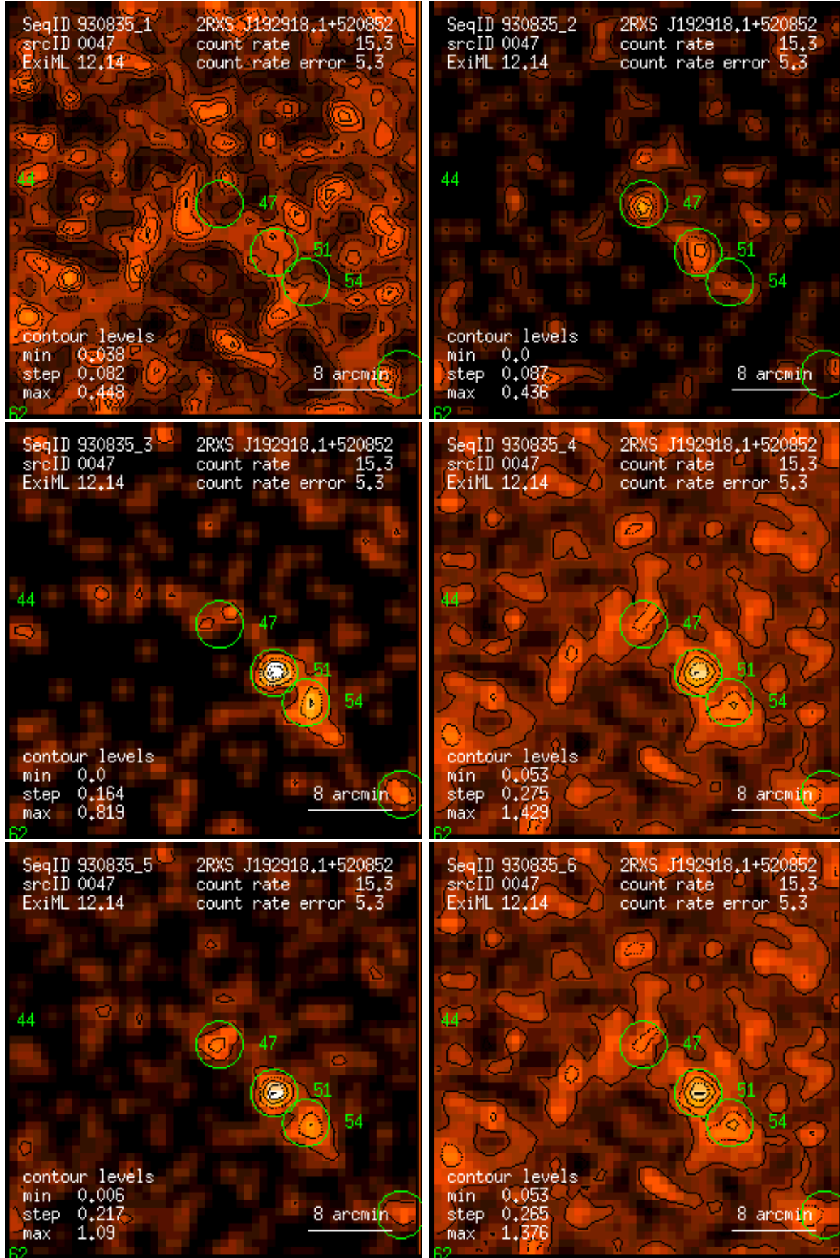
Figure 47: RASS 930835: detection 0047: band rate images, Gaussian filter: (1) PSPC channels 11 – 41, (2) 52 – 90, (3) 91 – 201, (4) 11 – 235, (5) 52 – 201, (6) 11 – 201. Broad band rates in counts/ks. Band rate contour levels in counts/ks/arcmin 2 .
