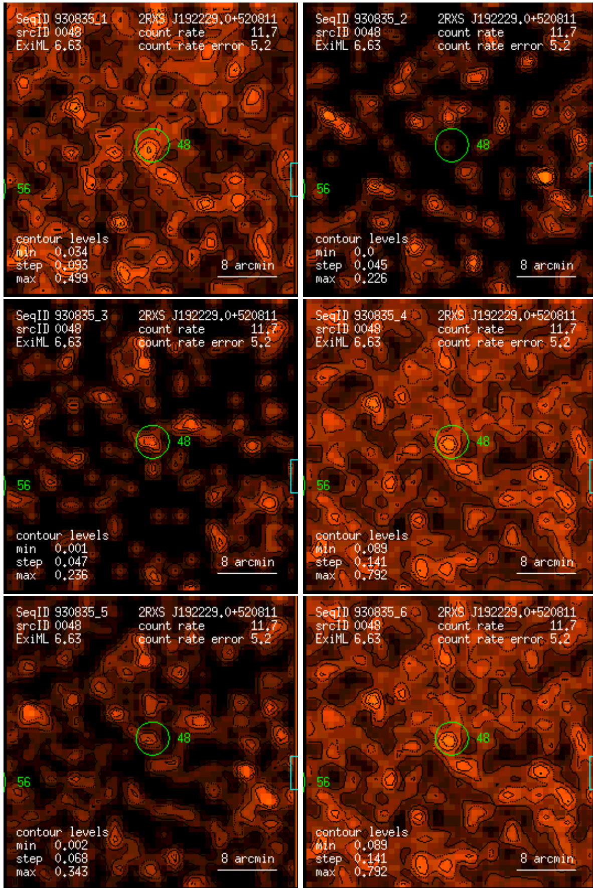
Figure 48: RASS 930835: detection 0048: band rate images, Gaussian filter: (1) PSPC channels 11 – 41, (2) 52 – 90, (3) 91 – 201, (4) 11 – 235, (5) 52 – 201, (6) 11 – 201. Broad band rates in counts/ks. Band rate contour levels in counts/ks/arcmin 2 .
