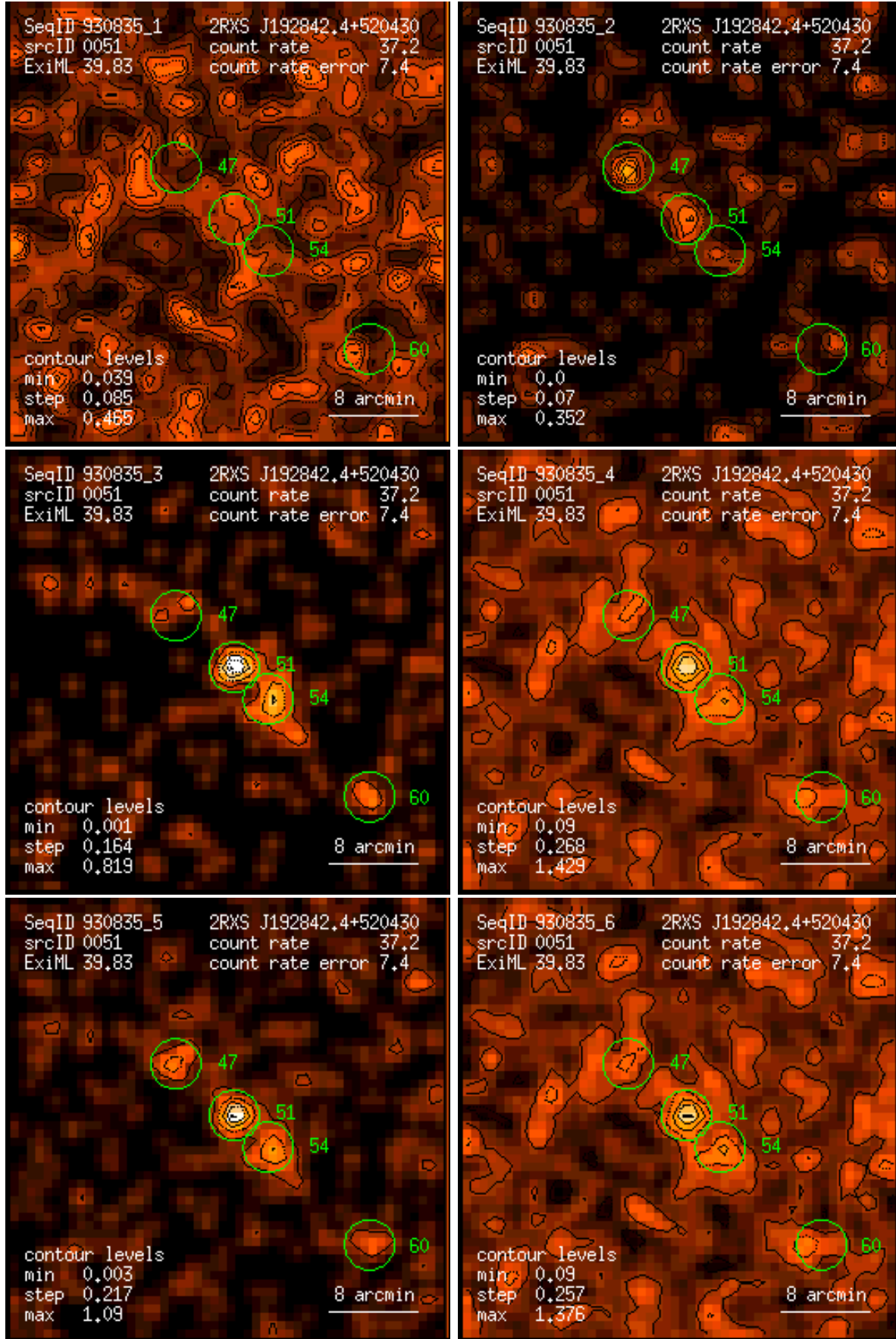
Figure 51: RASS 930835: detection 0051: band rate images, Gaussian filter: (1) PSPC channels 11 – 41, (2) 52 – 90, (3) 91 – 201, (4) 11 – 235, (5) 52 – 201, (6) 11 – 201. Broad band rates in counts/ks. Band rate contour levels in counts/ks/arcmin 2 .
