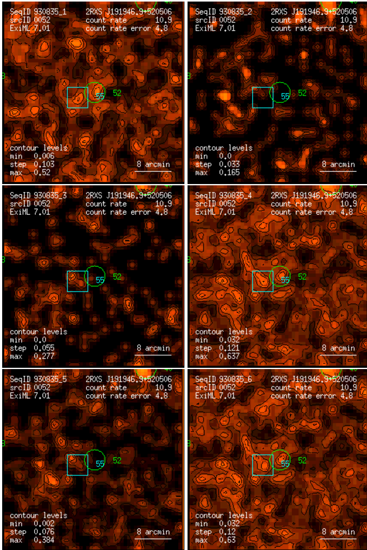
Figure 52: RASS 930835: detection 0052: band rate images, Gaussian filter: (1) PSPC channels 11 – 41, (2) 52 – 90, (3) 91 – 201, (4) 11 – 235, (5) 52 – 201, (6) 11 – 201. Broad band rates in counts/ks. Band rate contour levels in counts/ks/arcmin 2 .
