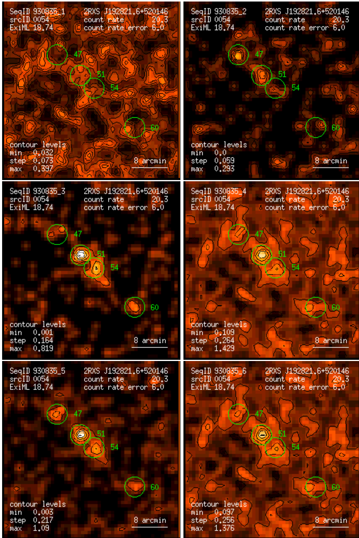
Figure 54: RASS 930835: detection 0054: band rate images, Gaussian filter: (1) PSPC channels 11 – 41, (2) 52 – 90, (3) 91 – 201, (4) 11 – 235, (5) 52 – 201, (6) 11 – 201. Broad band rates in counts/ks. Band rate contour levels in counts/ks/arcmin 2 .
