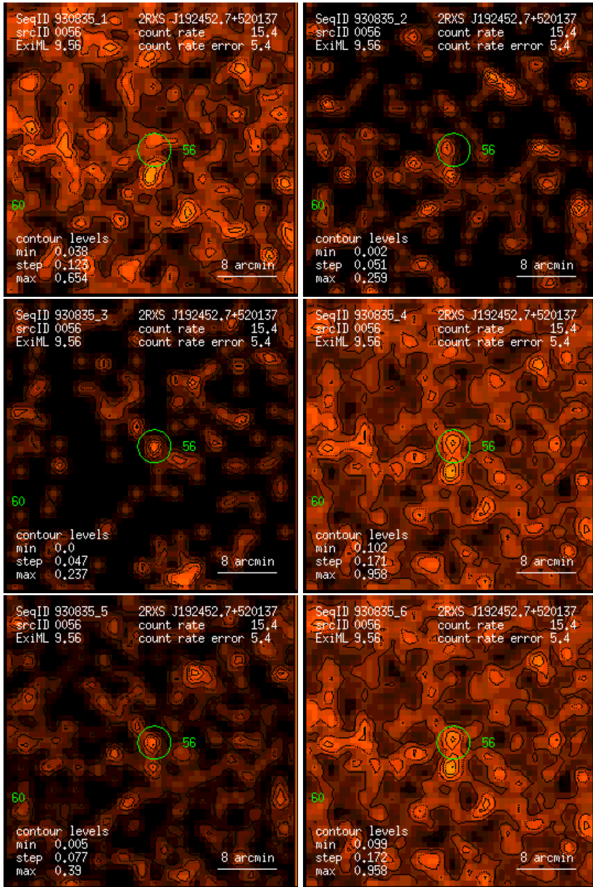
Figure 56: RASS 930835: detection 0056: band rate images, Gaussian filter: (1) PSPC channels 11 – 41, (2) 52 – 90, (3) 91 – 201, (4) 11 – 235, (5) 52 – 201, (6) 11 – 201. Broad band rates in counts/ks. Band rate contour levels in counts/ks/arcmin 2 .
