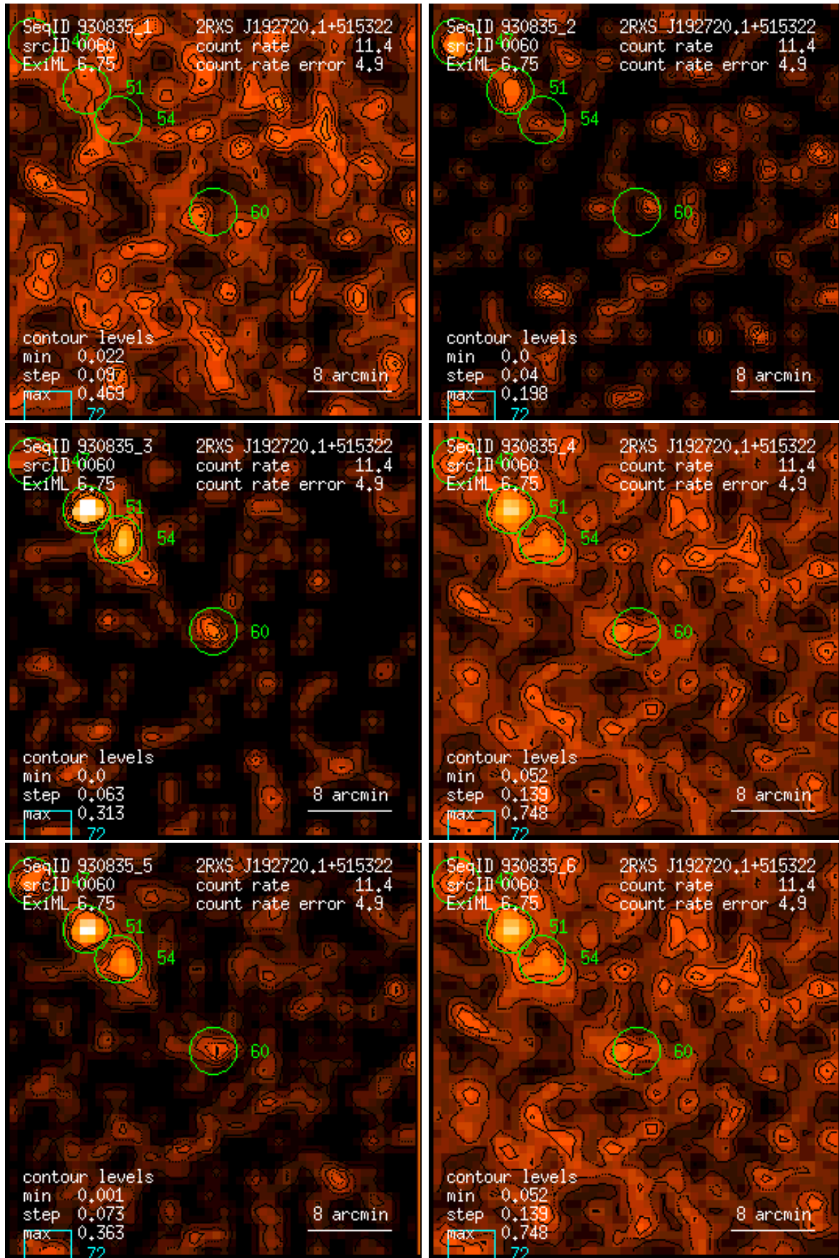
Figure 60: RASS 930835: detection 0060: band rate images, Gaussian filter: (1) PSPC channels 11 – 41, (2) 52 – 90, (3) 91 – 201, (4) 11 – 235, (5) 52 – 201, (6) 11 – 201. Broad band rates in counts/ks. Band rate contour levels in counts/ks/arcmin 2 .
