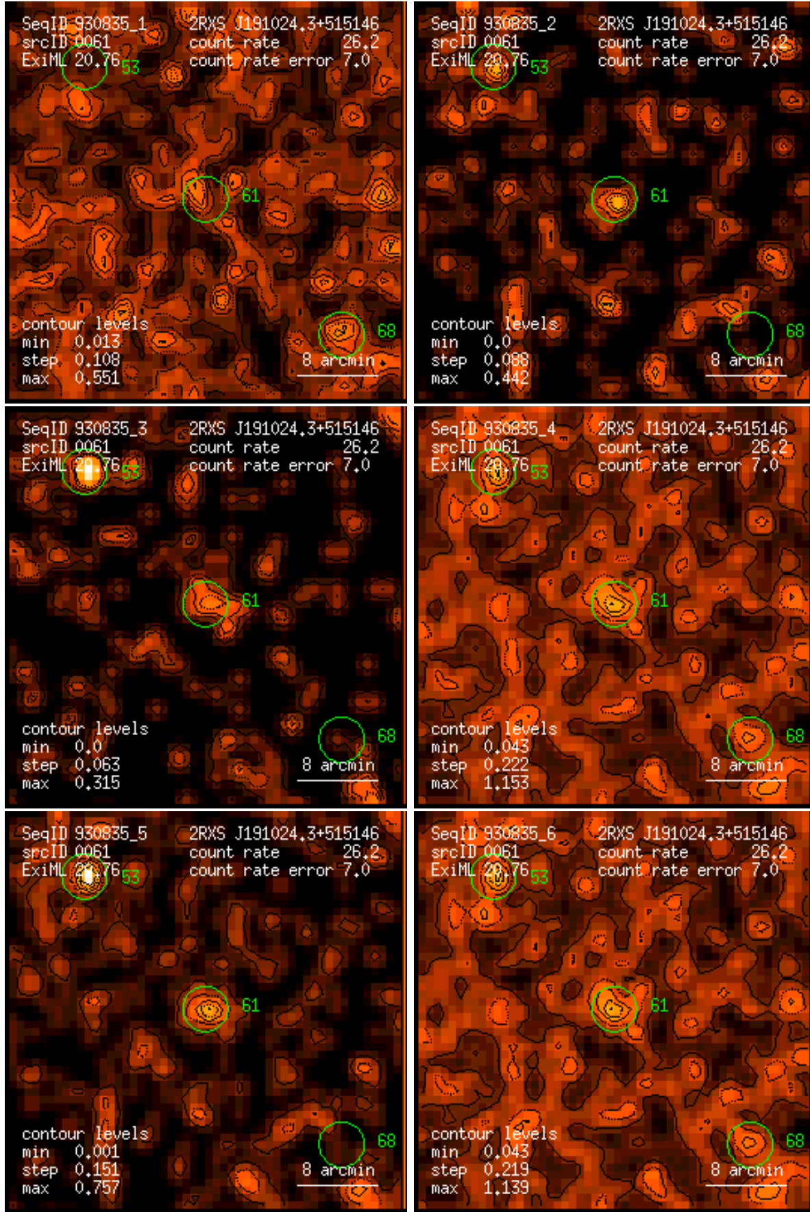
Figure 61: RASS 930835: detection 0061: band rate images, Gaussian filter: (1) PSPC channels 11 – 41, (2) 52 – 90, (3) 91 – 201, (4) 11 – 235, (5) 52 – 201, (6) 11 – 201. Broad band rates in counts/ks. Band rate contour levels in counts/ks/arcmin 2 .
