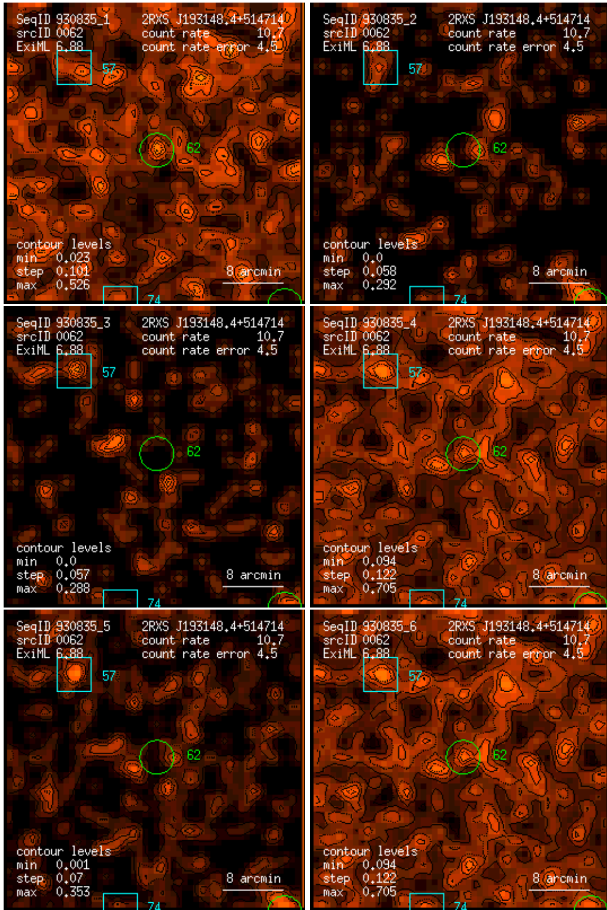
Figure 62: RASS 930835: detection 0062: band rate images, Gaussian filter: (1) PSPC channels 11 – 41, (2) 52 – 90, (3) 91 – 201, (4) 11 – 235, (5) 52 – 201, (6) 11 – 201. Broad band rates in counts/ks. Band rate contour levels in counts/ks/arcmin 2 .
