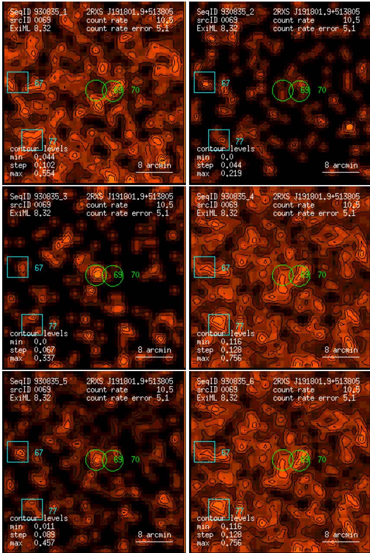
Figure 69: RASS 930835: detection 0069: band rate images, Gaussian filter: (1) PSPC channels 11 – 41, (2) 52 – 90, (3) 91 – 201, (4) 11 – 235, (5) 52 – 201, (6) 11 – 201. Broad band rates in counts/ks. Band rate contour levels in counts/ks/arcmin 2 .
