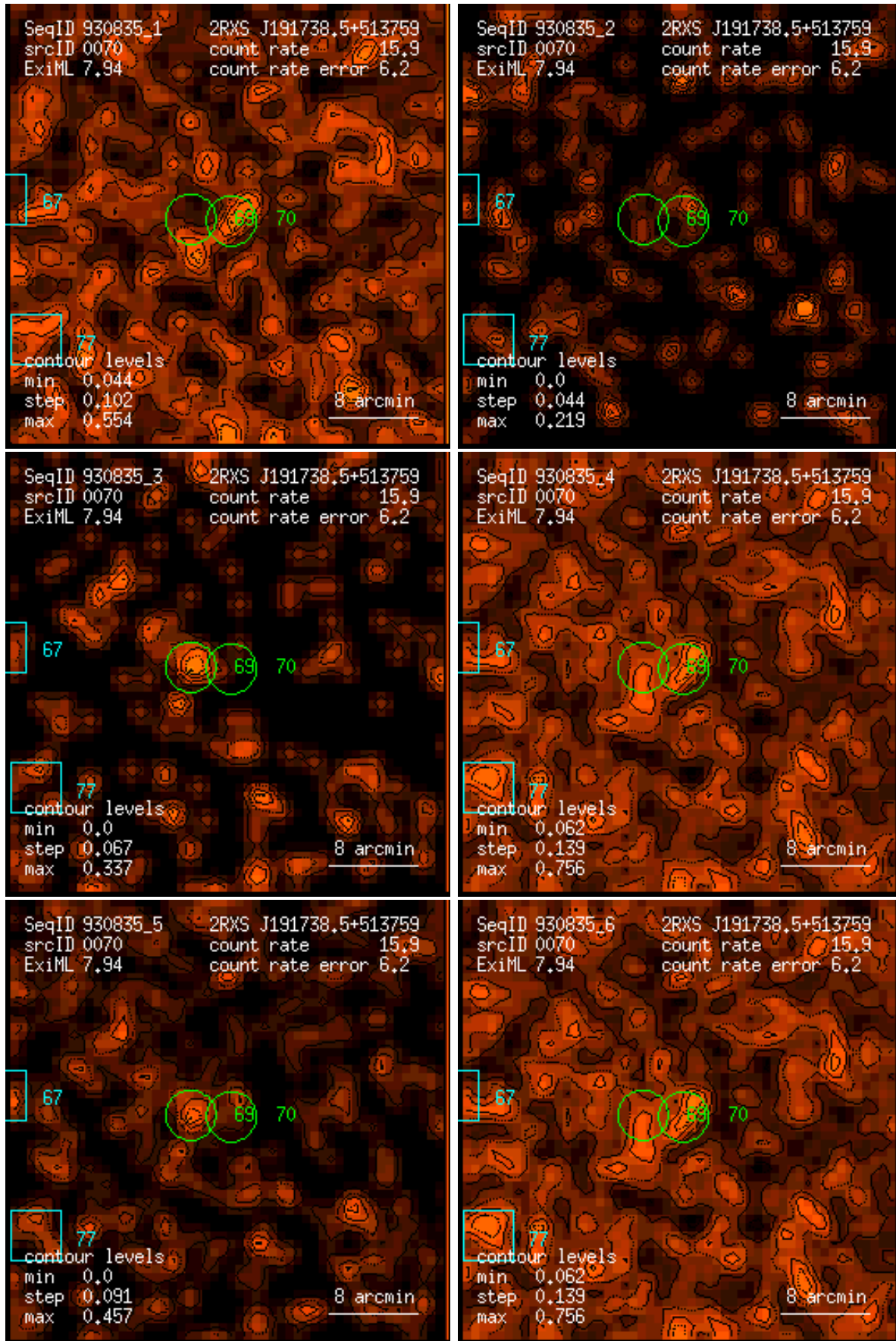
Figure 70: RASS 930835: detection 0070: band rate images, Gaussian filter: (1) PSPC channels 11 – 41, (2) 52 – 90, (3) 91 – 201, (4) 11 – 235, (5) 52 – 201, (6) 11 – 201. Broad band rates in counts/ks. Band rate contour levels in counts/ks/arcmin 2 .
