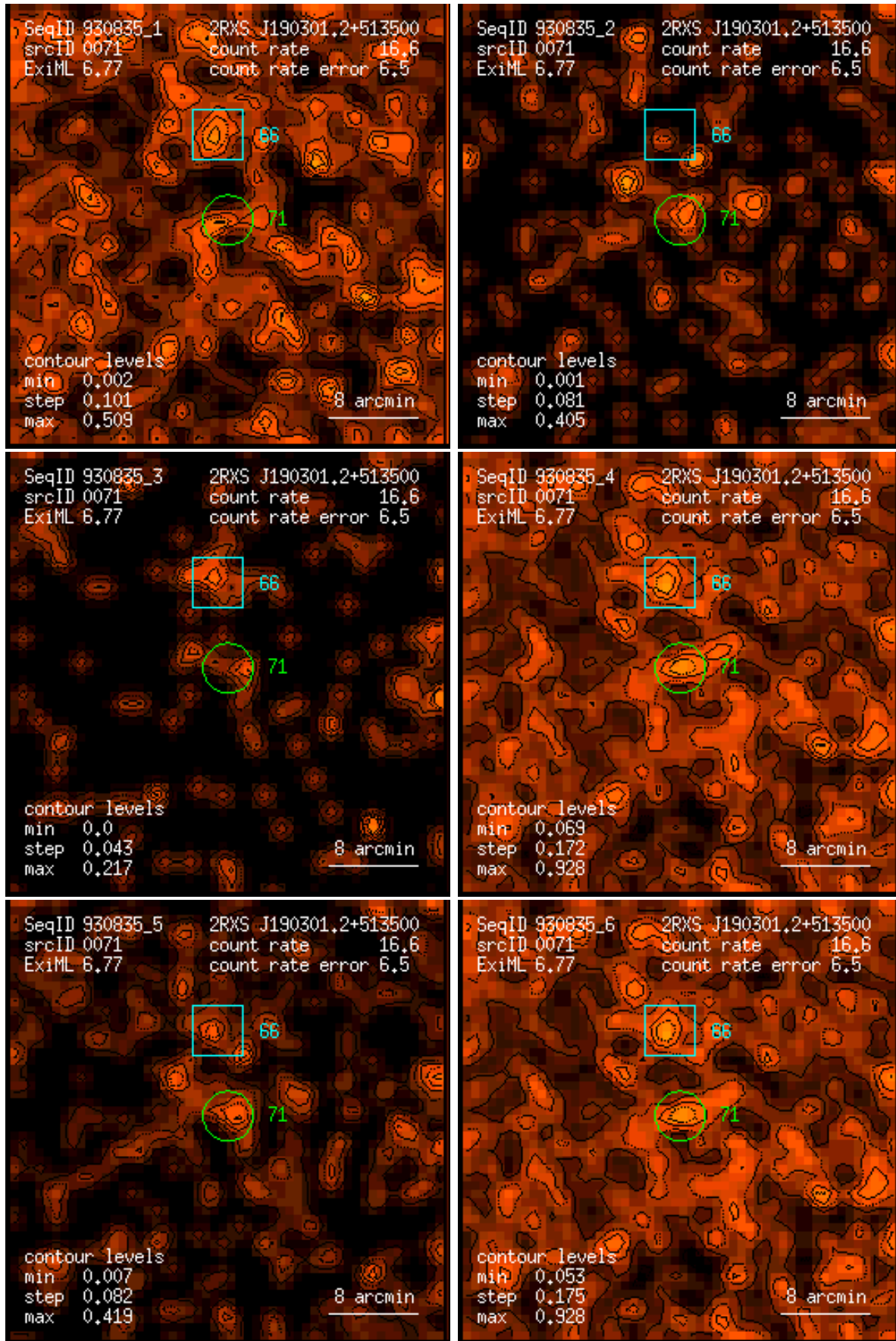
Figure 71: RASS 930835: detection 0071: band rate images, Gaussian filter: (1) PSPC channels 11 – 41, (2) 52 – 90, (3) 91 – 201, (4) 11 – 235, (5) 52 – 201, (6) 11 – 201. Broad band rates in counts/ks. Band rate contour levels in counts/ks/arcmin 2 .
