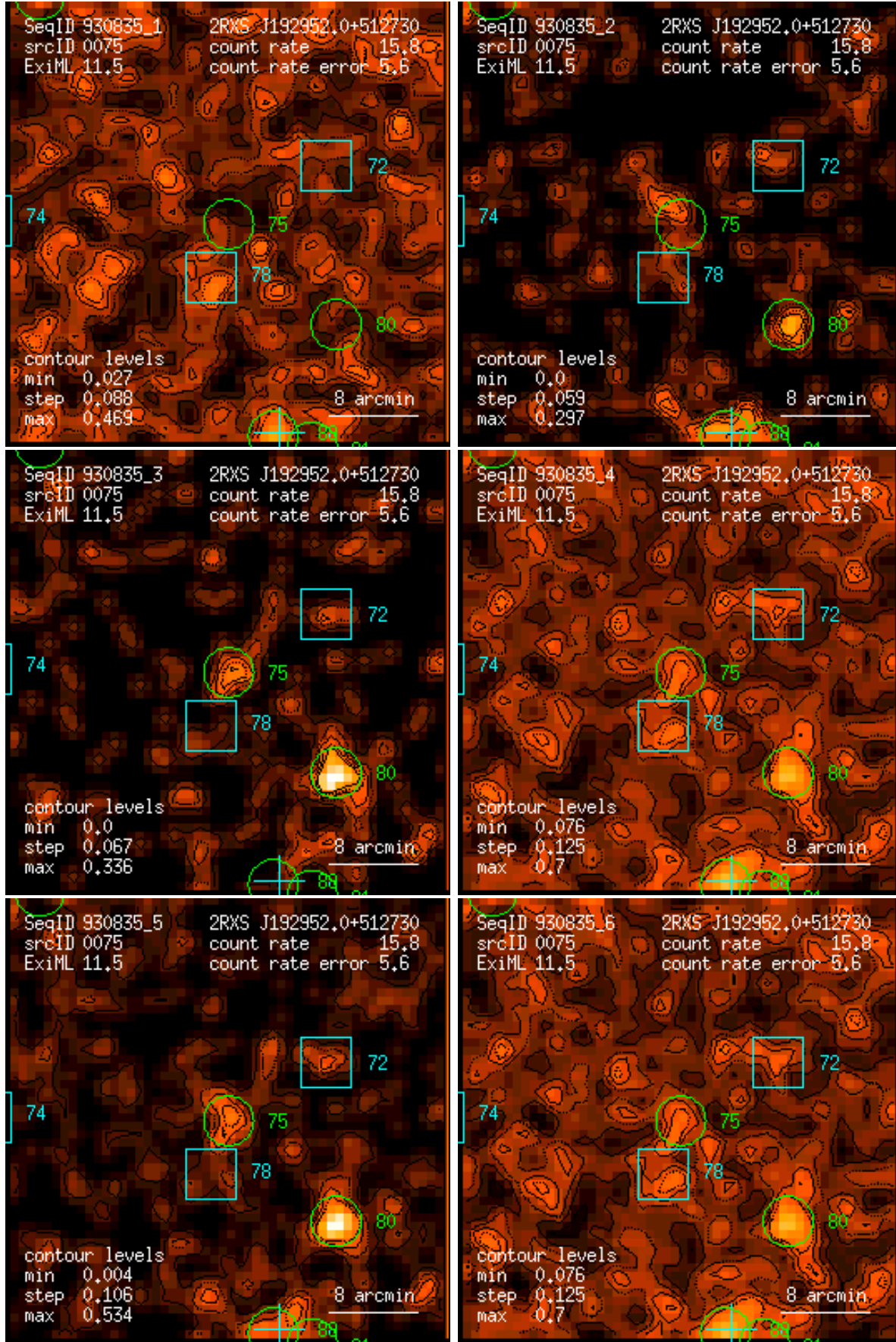
Figure 75: RASS 930835: detection 0075: band rate images, Gaussian filter: (1) PSPC channels 11 – 41, (2) 52 – 90, (3) 91 – 201, (4) 11 – 235, (5) 52 – 201, (6) 11 – 201. Broad band rates in counts/ks. Band rate contour levels in counts/ks/arcmin 2 .
