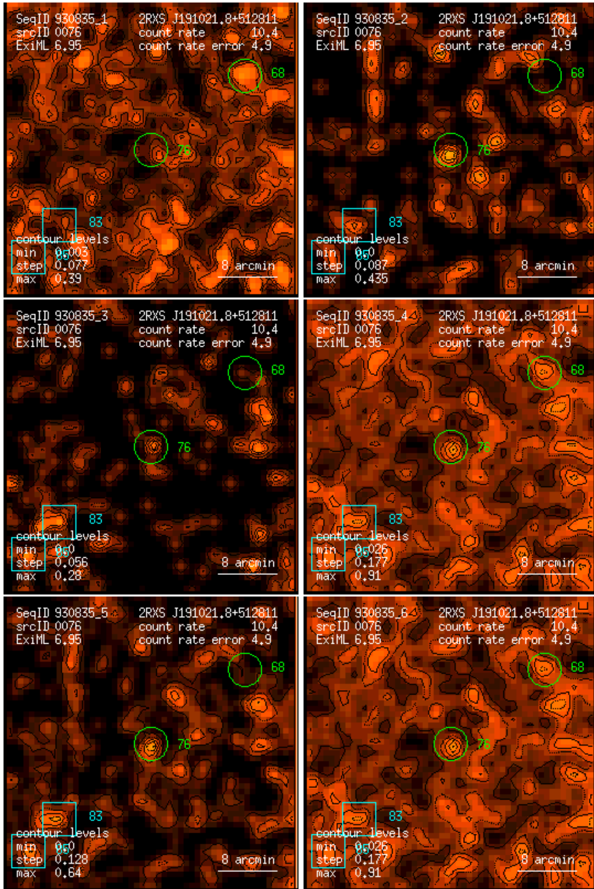
Figure 76: RASS 930835: detection 0076: band rate images, Gaussian filter: (1) PSPC channels 11 – 41, (2) 52 – 90, (3) 91 – 201, (4) 11 – 235, (5) 52 – 201, (6) 11 – 201. Broad band rates in counts/ks. Band rate contour levels in counts/ks/arcmin 2 .
