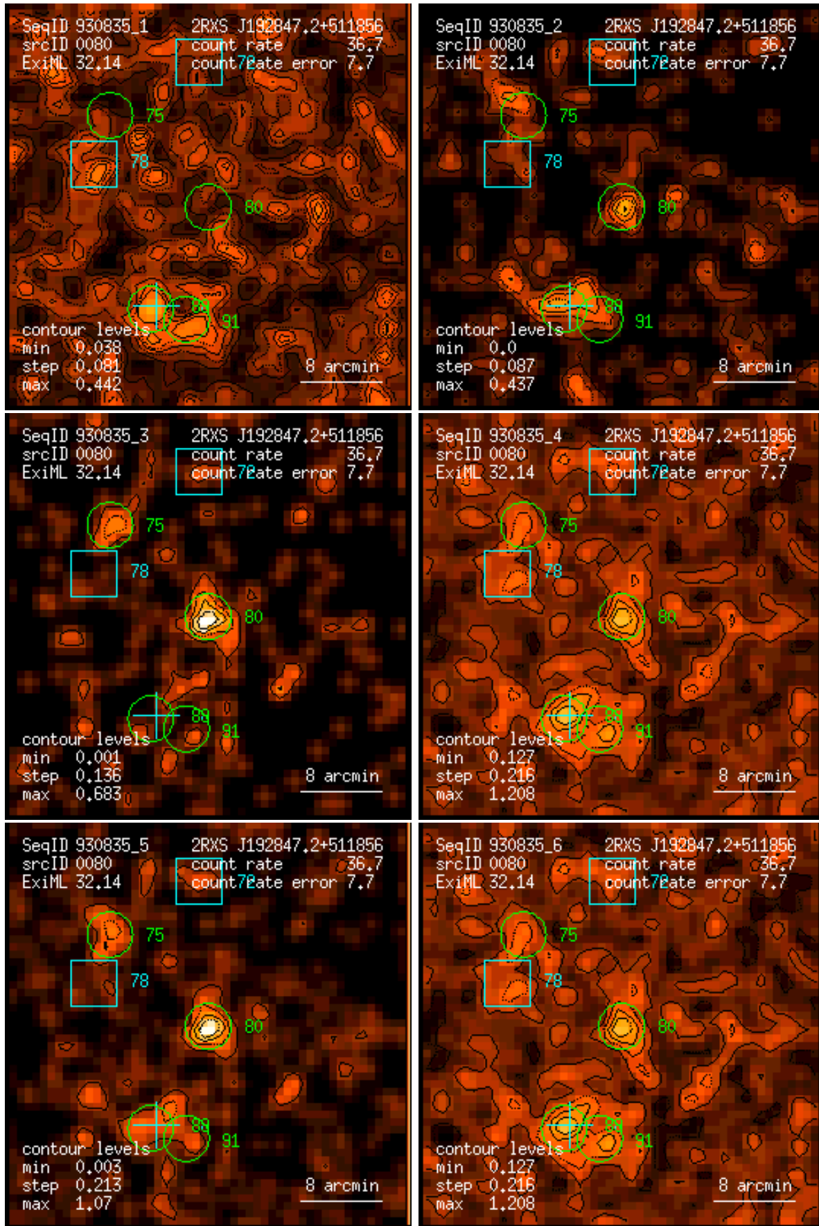
Figure 80: RASS 930835: detection 0080: band rate images, Gaussian filter: (1) PSPC channels 11 – 41, (2) 52 – 90, (3) 91 – 201, (4) 11 – 235, (5) 52 – 201, (6) 11 – 201. Broad band rates in counts/ks. Band rate contour levels in counts/ks/arcmin 2 .
