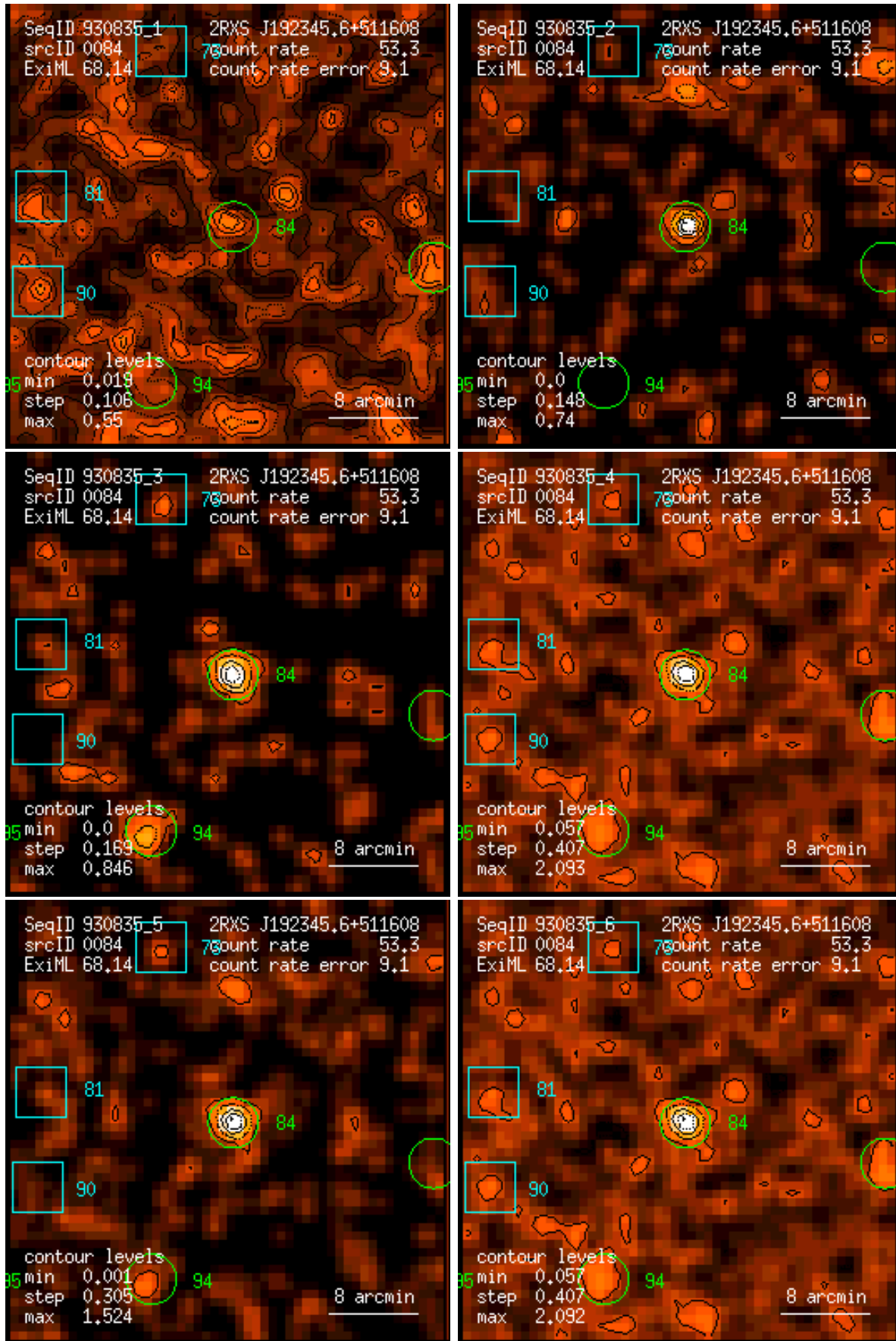
Figure 84: RASS 930835: detection 0084: band rate images, Gaussian filter: (1) PSPC channels 11 – 41, (2) 52 – 90, (3) 91 – 201, (4) 11 – 235, (5) 52 – 201, (6) 11 – 201. Broad band rates in counts/ks. Band rate contour levels in counts/ks/arcmin 2 .
