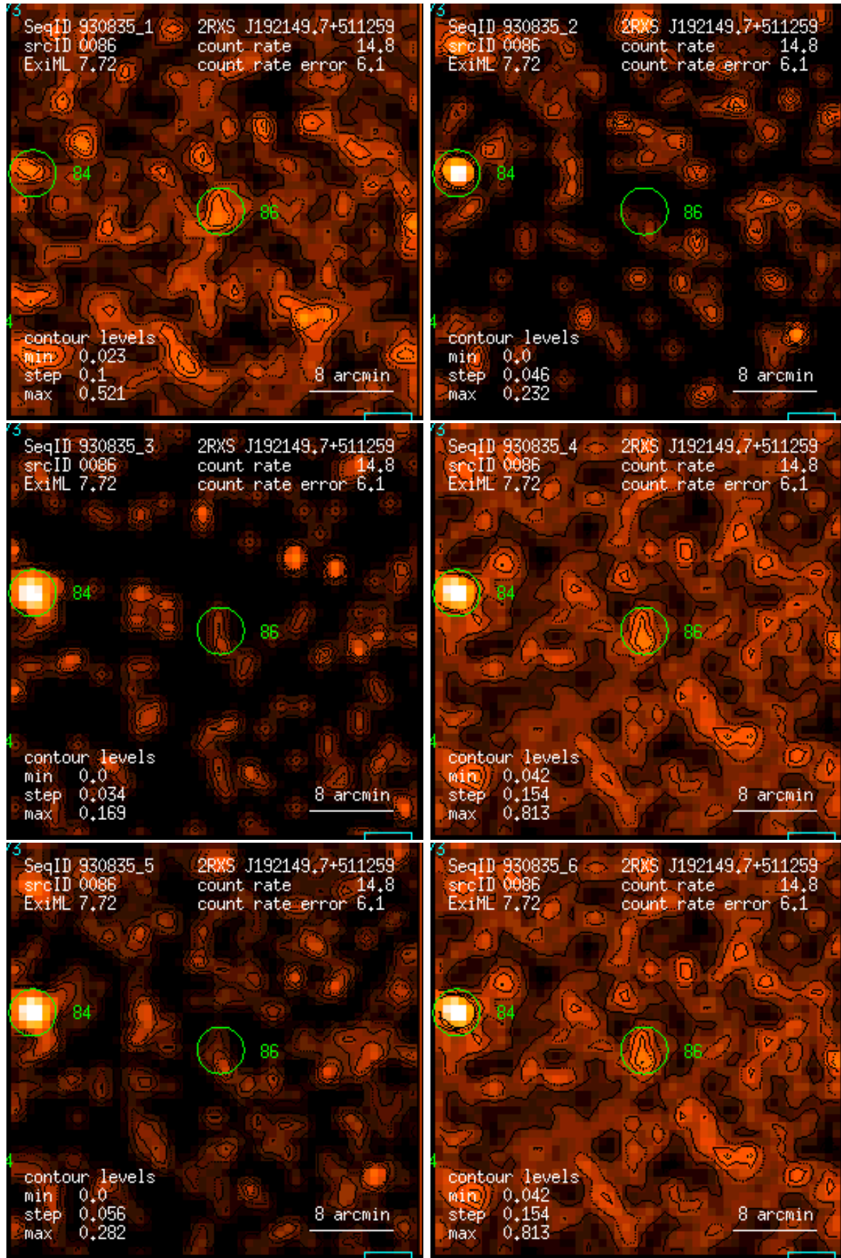
Figure 86: RASS 930835: detection 0086: band rate images, Gaussian filter: (1) PSPC channels 11 – 41, (2) 52 – 90, (3) 91 – 201, (4) 11 – 235, (5) 52 – 201, (6) 11 – 201. Broad band rates in counts/ks. Band rate contour levels in counts/ks/arcmin 2 .
