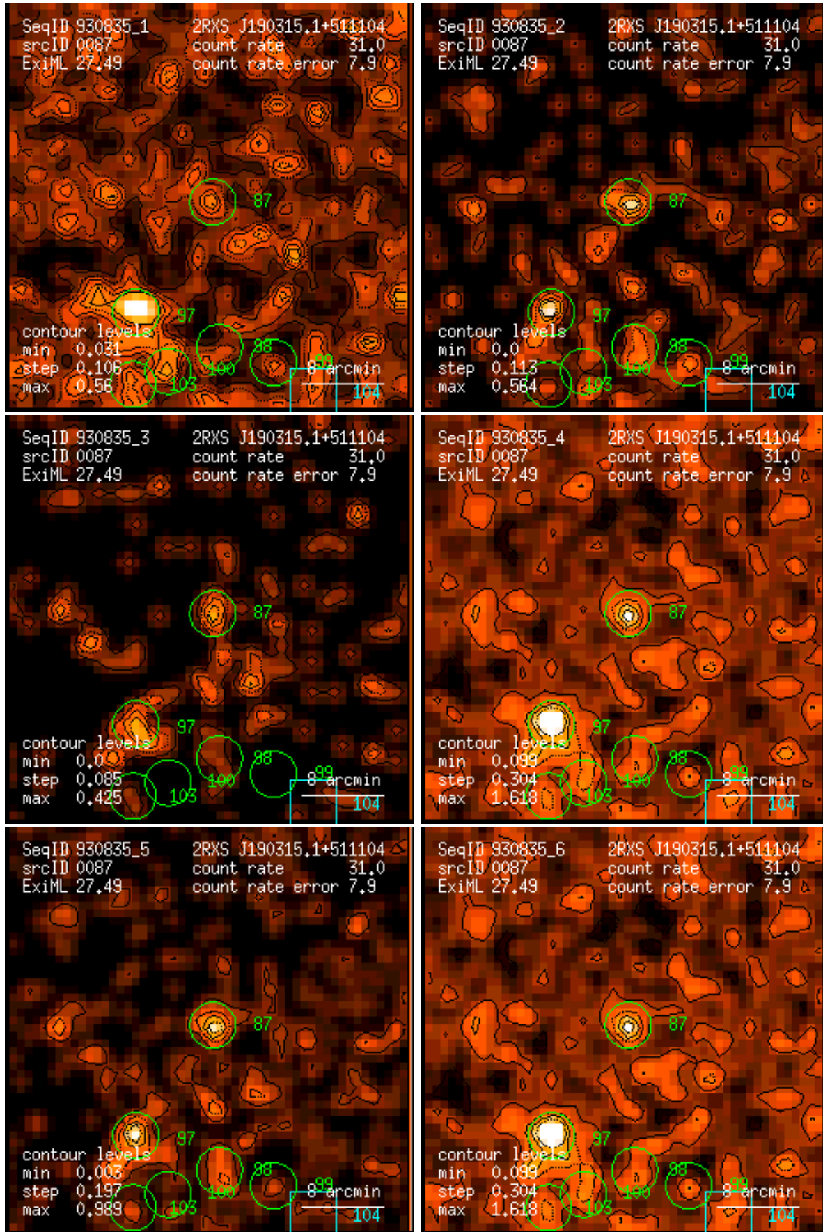
Figure 87: RASS 930835: detection 0087: band rate images, Gaussian filter: (1) PSPC channels 11 – 41, (2) 52 – 90, (3) 91 – 201, (4) 11 – 235, (5) 52 – 201, (6) 11 – 201. Broad band rates in counts/ks. Band rate contour levels in counts/ks/arcmin 2 .
