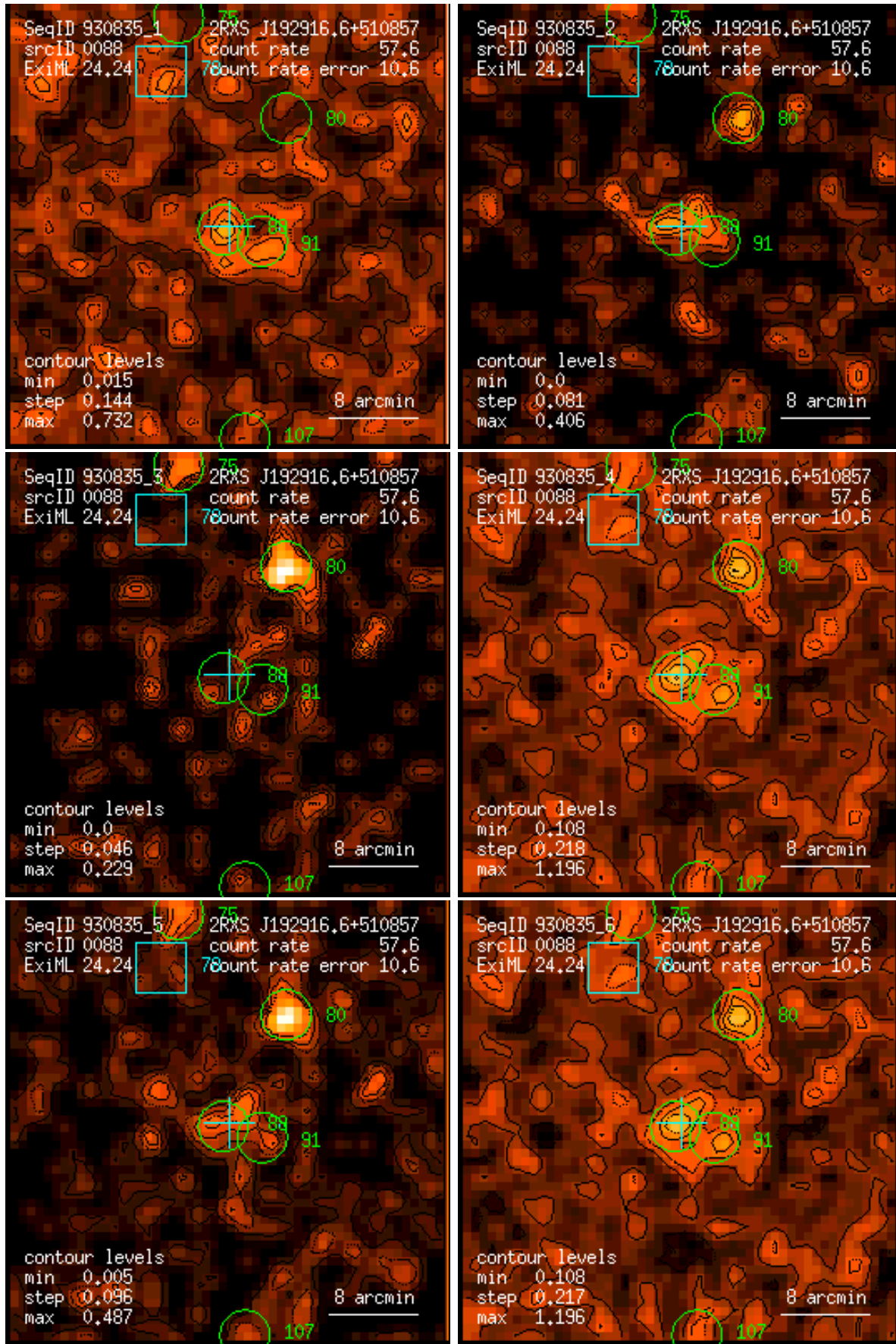
Figure 88: RASS 930835: detection 0088: band rate images, Gaussian filter: (1) PSPC channels 11 – 41, (2) 52 – 90, (3) 91 – 201, (4) 11 – 235, (5) 52 – 201, (6) 11 – 201. Broad band rates in counts/ks. Band rate contour levels in counts/ks/arcmin 2 .
