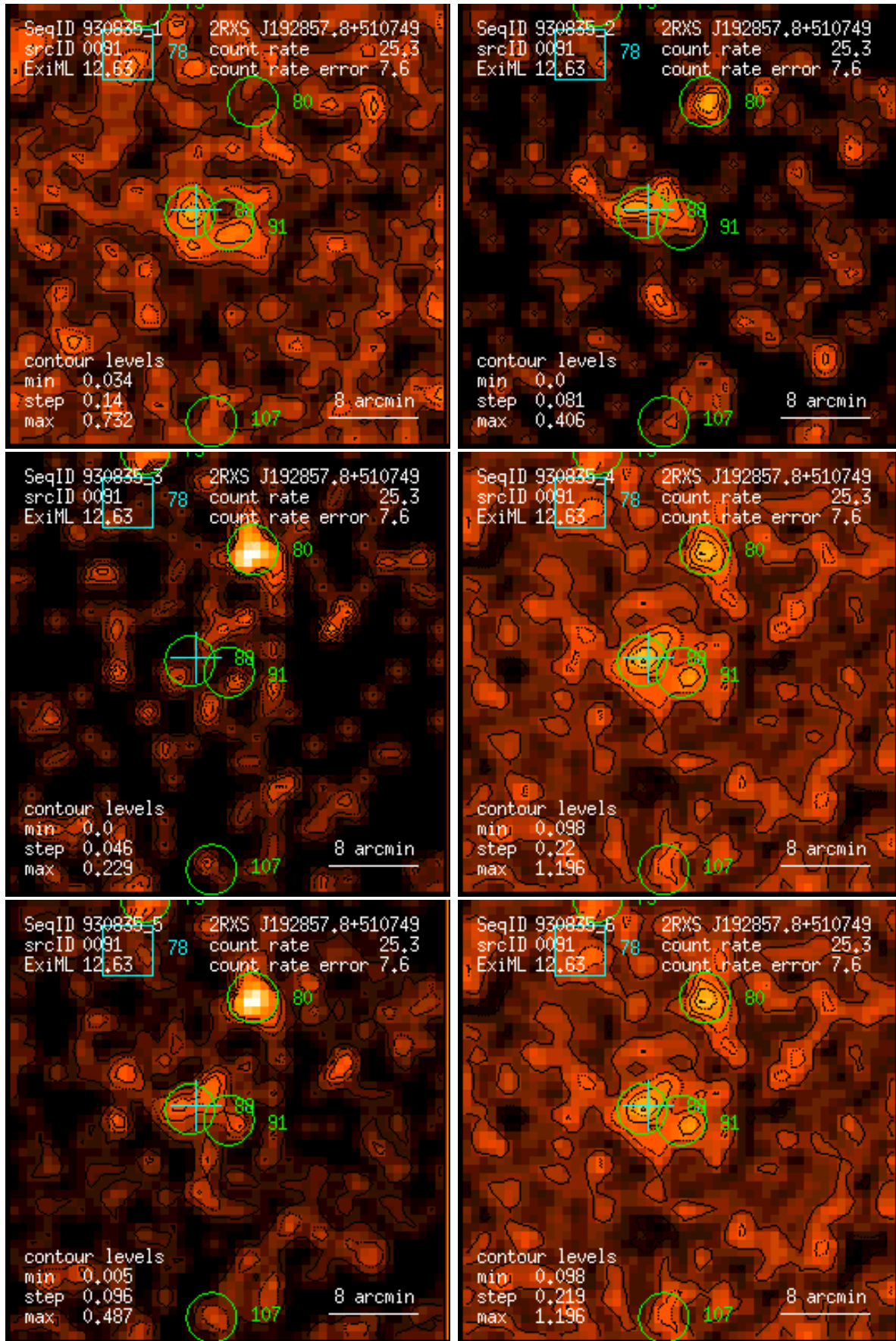
Figure 91: RASS 930835: detection 0091: band rate images, Gaussian filter: (1) PSPC channels 11 – 41, (2) 52 – 90, (3) 91 – 201, (4) 11 – 235, (5) 52 – 201, (6) 11 – 201. Broad band rates in counts/ks. Band rate contour levels in counts/ks/arcmin 2 .
