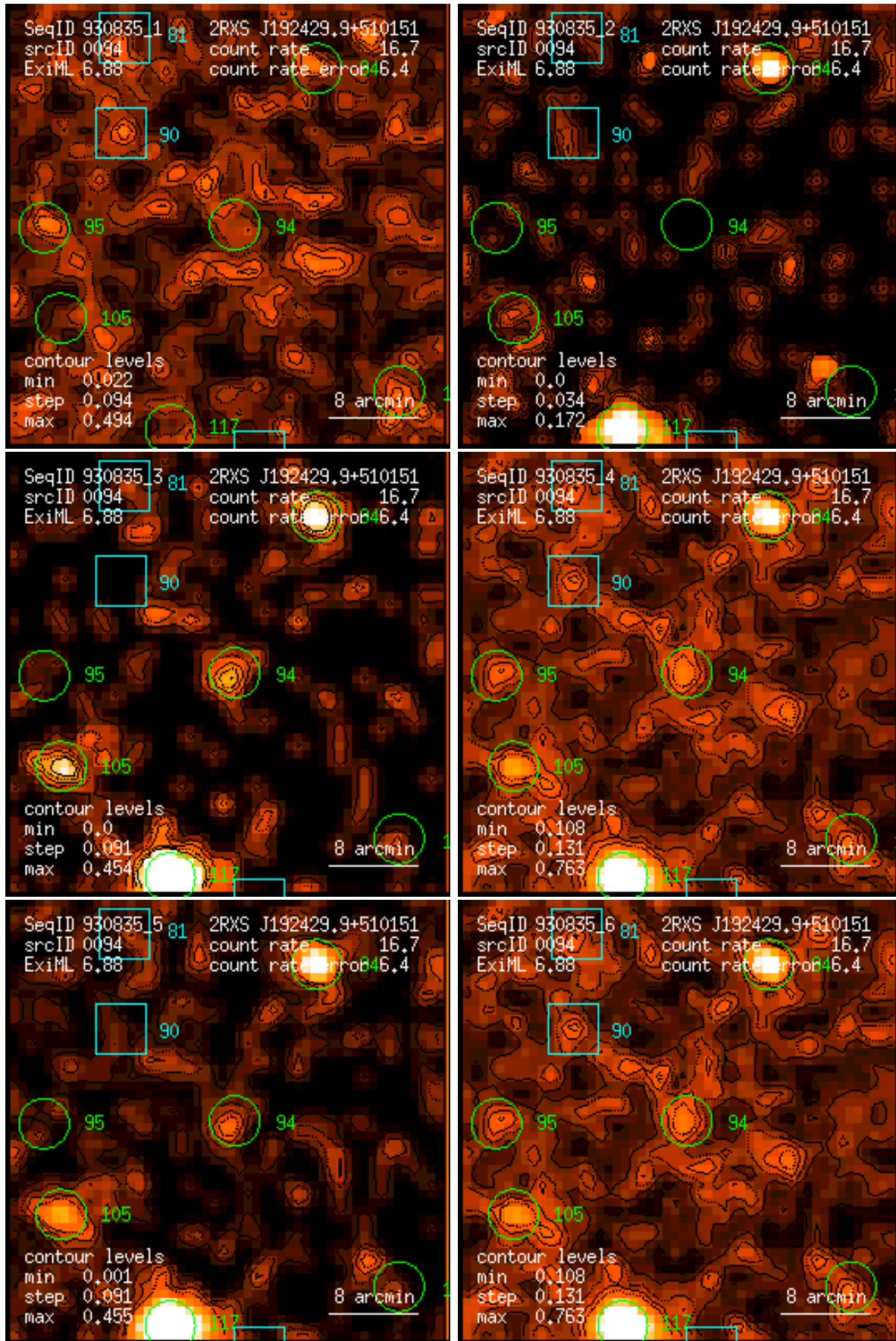
Figure 94: RASS 930835: detection 0094: band rate images, Gaussian filter: (1) PSPC channels 11 – 41, (2) 52 – 90, (3) 91 – 201, (4) 11 – 235, (5) 52 – 201, (6) 11 – 201. Broad band rates in counts/ks. Band rate contour levels in counts/ks/arcmin 2 .
