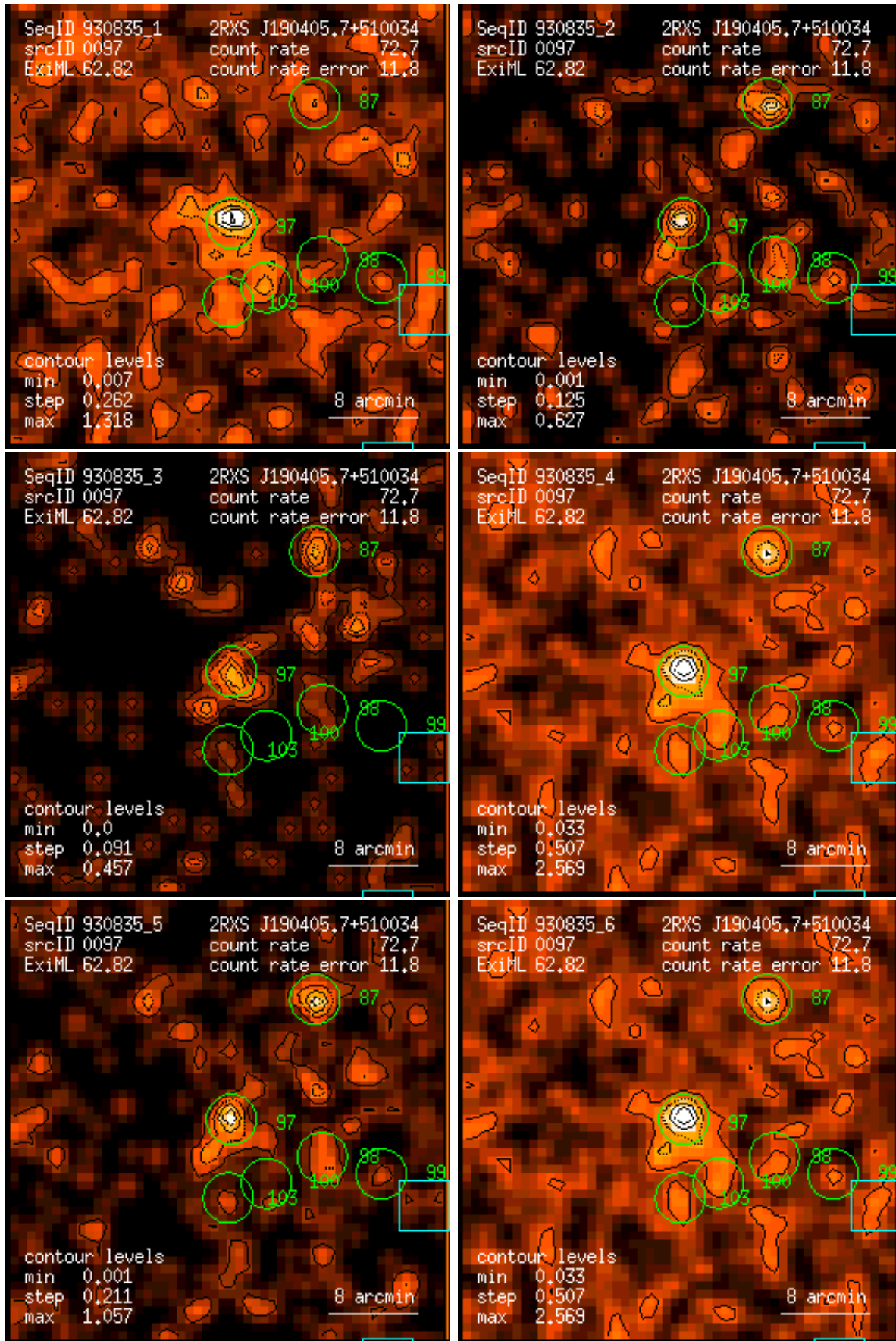
Figure 97: RASS 930835: detection 0097: band rate images, Gaussian filter: (1) PSPC channels 11 – 41, (2) 52 – 90, (3) 91 – 201, (4) 11 – 235, (5) 52 – 201, (6) 11 – 201. Broad band rates in counts/ks. Band rate contour levels in counts/ks/arcmin 2 .
