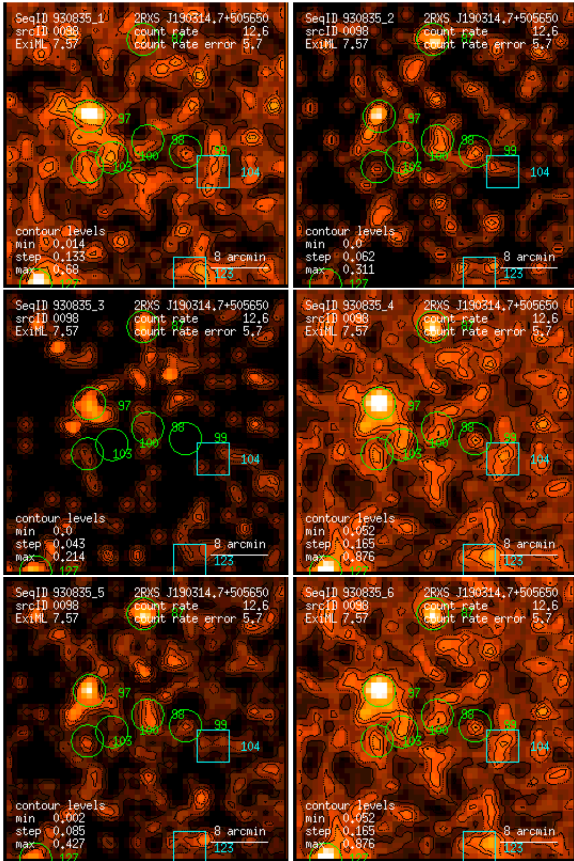
Figure 98: RASS 930835: detection 0098: band rate images, Gaussian filter: (1) PSPC channels 11 – 41, (2) 52 – 90, (3) 91 – 201, (4) 11 – 235, (5) 52 – 201, (6) 11 – 201. Broad band rates in counts/ks. Band rate contour levels in counts/ks/arcmin 2 .
