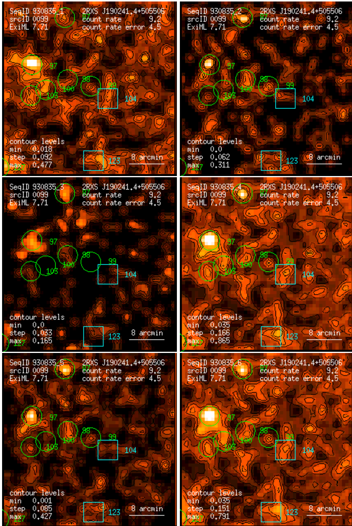
Figure 99: RASS 930835: detection 0099: band rate images, Gaussian filter: (1) PSPC channels 11 – 41, (2) 52 – 90, (3) 91 – 201, (4) 11 – 235, (5) 52 – 201, (6) 11 – 201. Broad band rates in counts/ks. Band rate contour levels in counts/ks/arcmin 2 .
