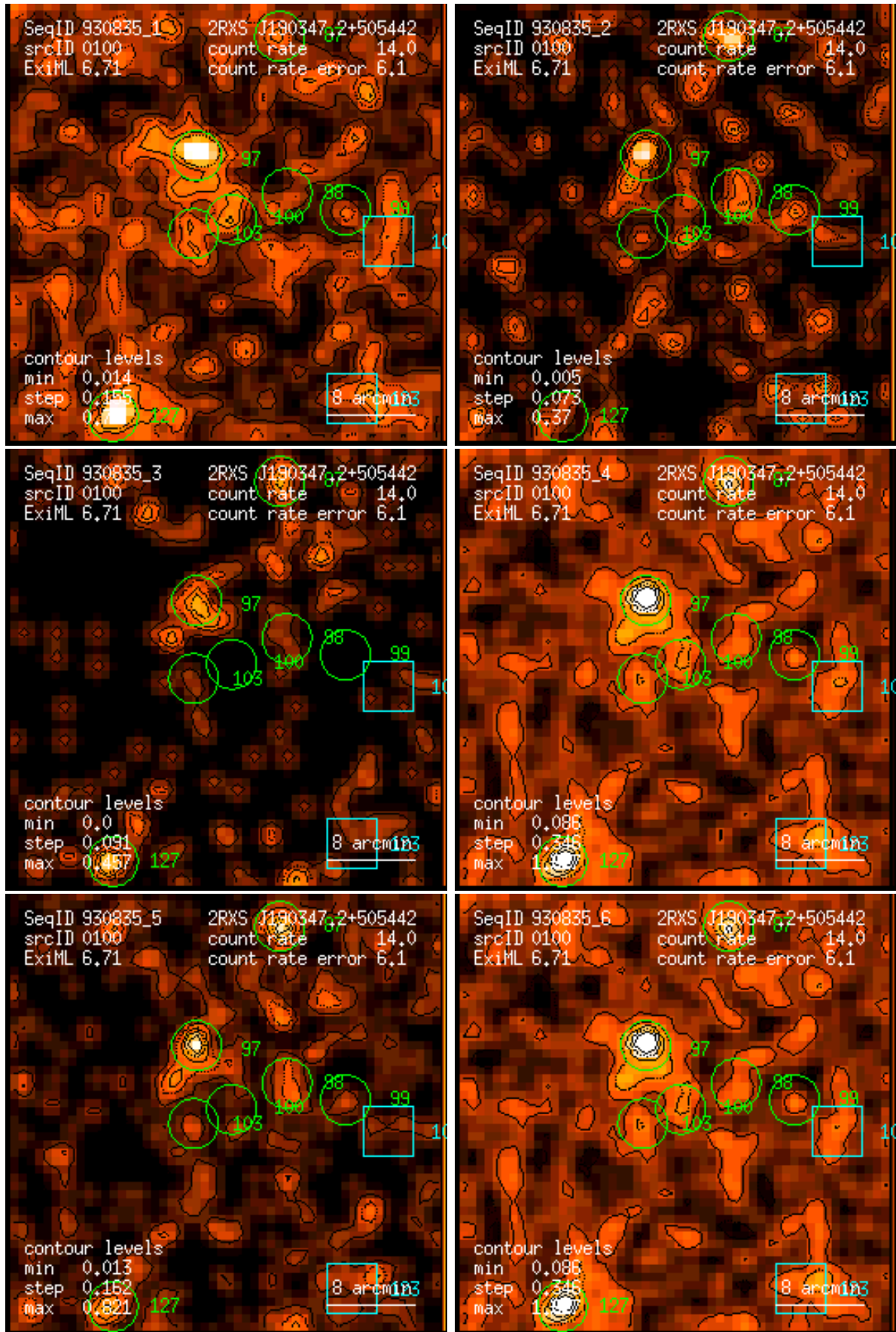
Figure 100: RASS 930835: detection 0100: band rate images, Gaussian filter: (1) PSPC channels 11 – 41, (2) 52 – 90, (3) 91 – 201, (4) 11 – 235, (5) 52 – 201, (6) 11 – 201. Broad band rates in counts/ks. Band rate contour levels in counts/ks/arcmin 2 .
