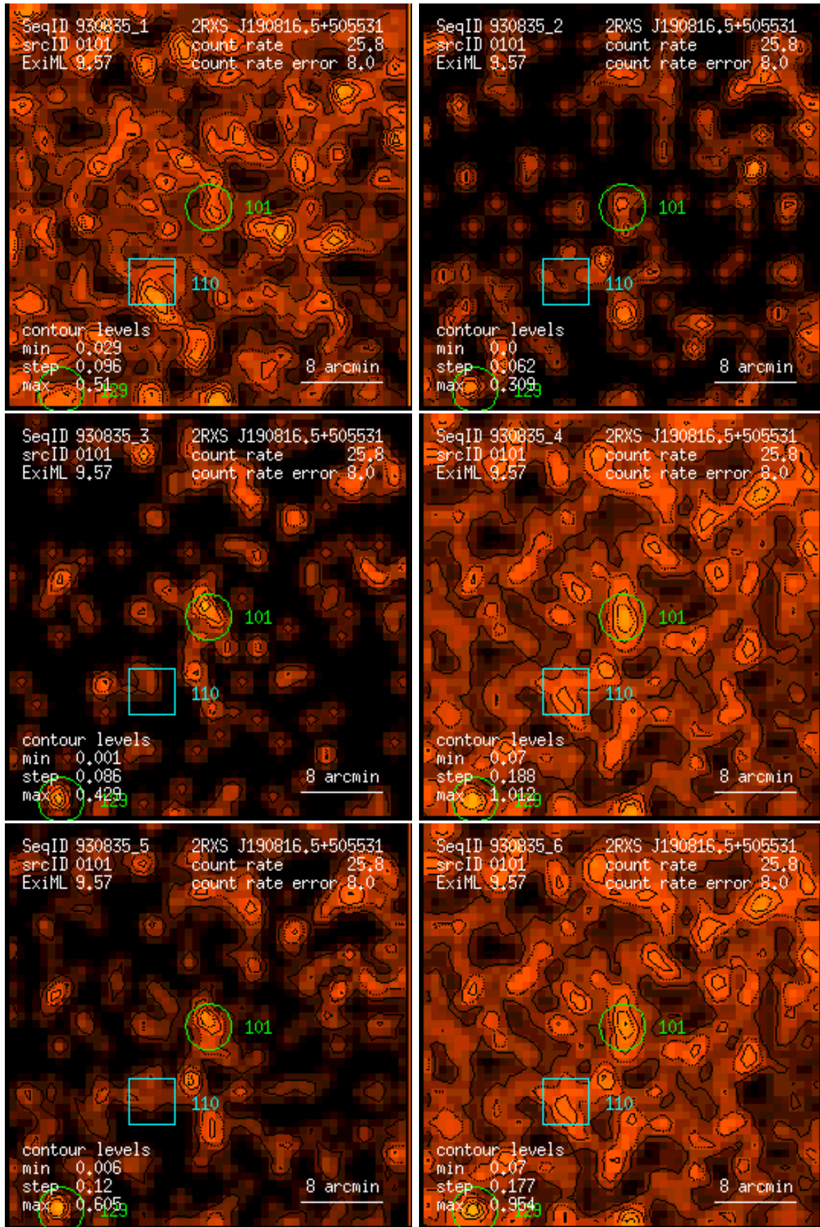
Figure 101: RASS 930835: detection 0101: band rate images, Gaussian filter: (1) PSPC channels 11 – 41, (2) 52 – 90, (3) 91 – 201, (4) 11 – 235, (5) 52 – 201, (6) 11 – 201. Broad band rates in counts/ks. Band rate contour levels in counts/ks/arcmin 2 .
