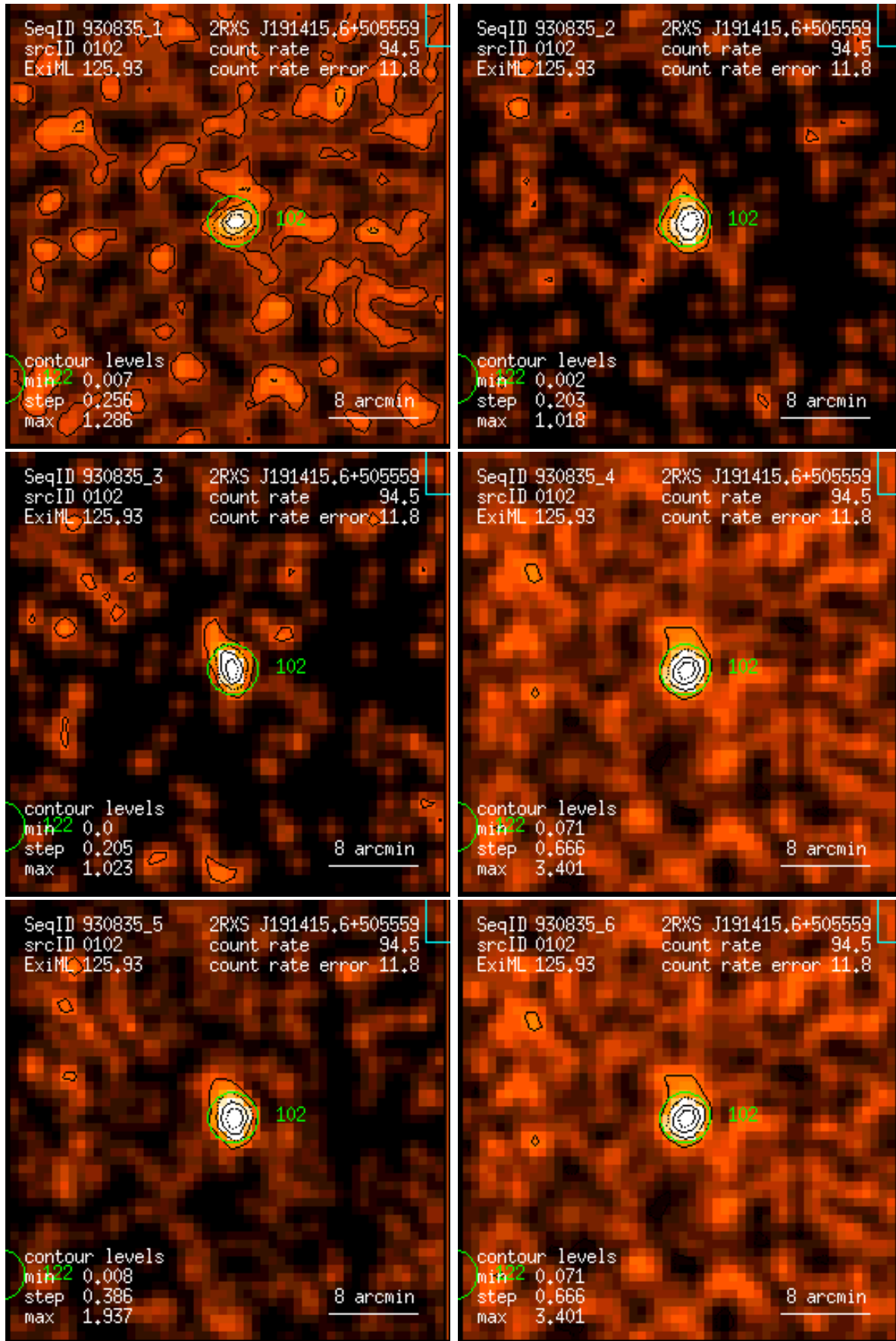
Figure 102: RASS 930835: detection 0102: band rate images, Gaussian filter: (1) PSPC channels 11 – 41, (2) 52 – 90, (3) 91 – 201, (4) 11 – 235, (5) 52 – 201, (6) 11 – 201. Broad band rates in counts/ks. Band rate contour levels in counts/ks/arcmin 2 .
